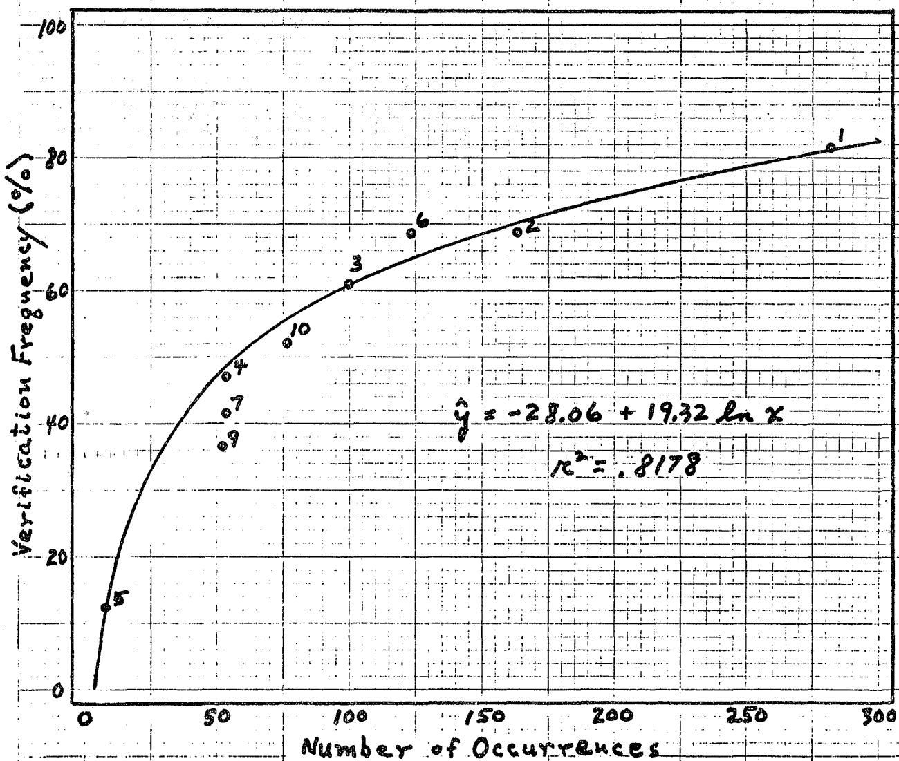
Figure 1. Verification frequency as a function of the frequency with which a map type occurs. Numbers with plotted points are winter map type.
