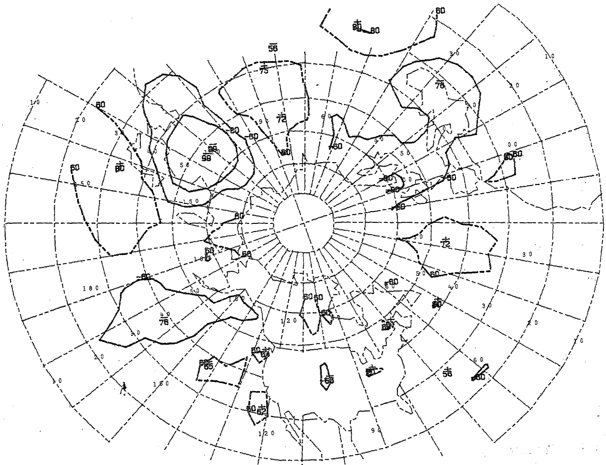
- KEY AT130E 50N 20 CASES
