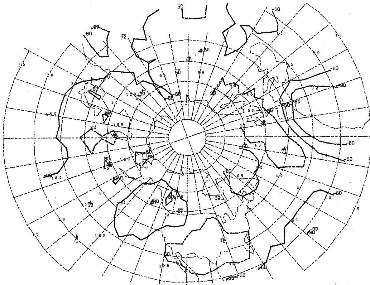
= KEY AT 10W 30N 19 CASES
