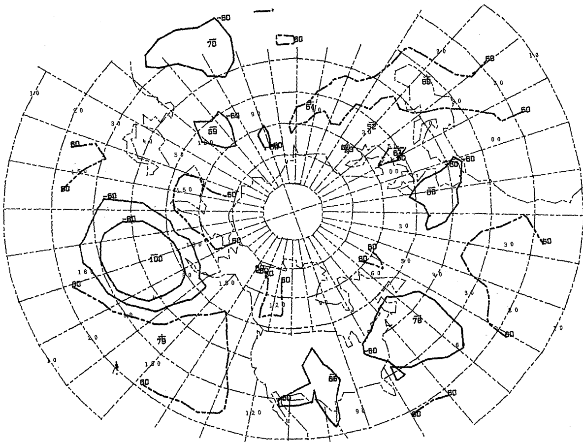
- KEY AT180 40N 25 CASES
