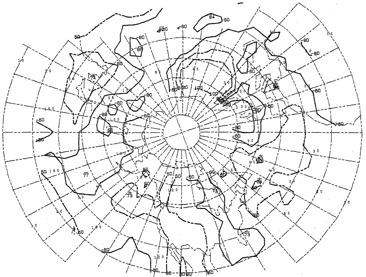
+ KEY AT 50E 60N 09 CASES
