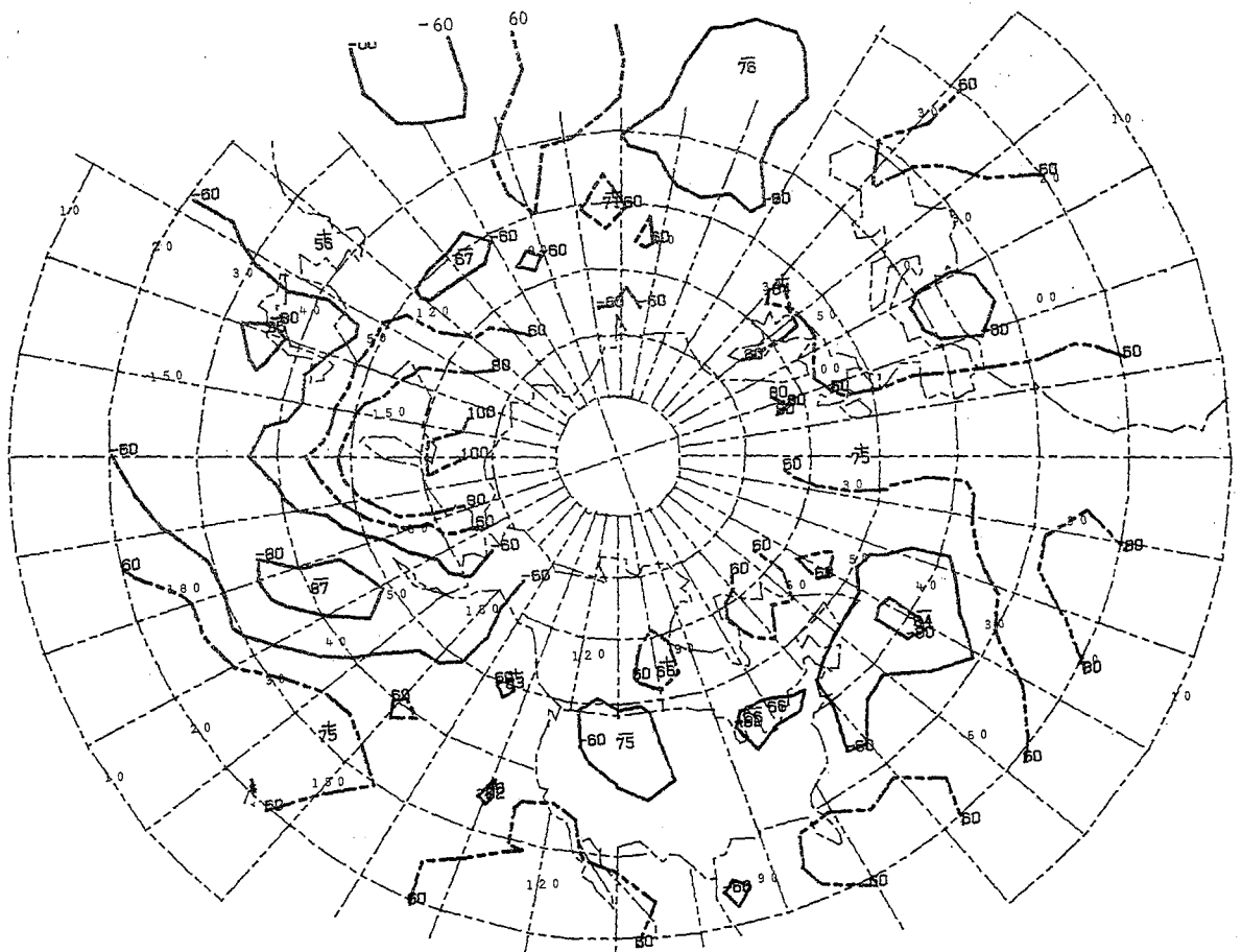
± KEY AT160E 60N 10 CASES
