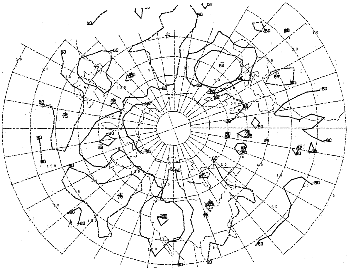
KEY AT 40E 50N 10 CASES
