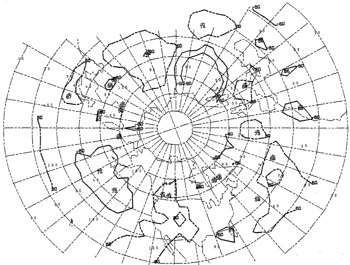
- KEY AT 50E 60N 14 CASES
