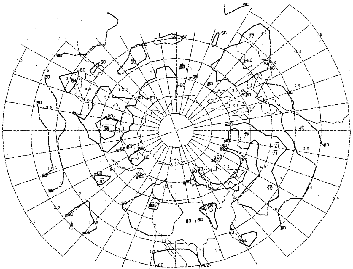
+ KEY AT 60W 60N 12 CASES
