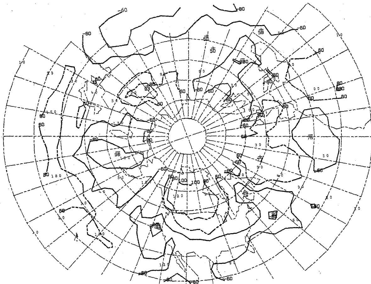
+ KEY AT110W 60N 09 CASES
