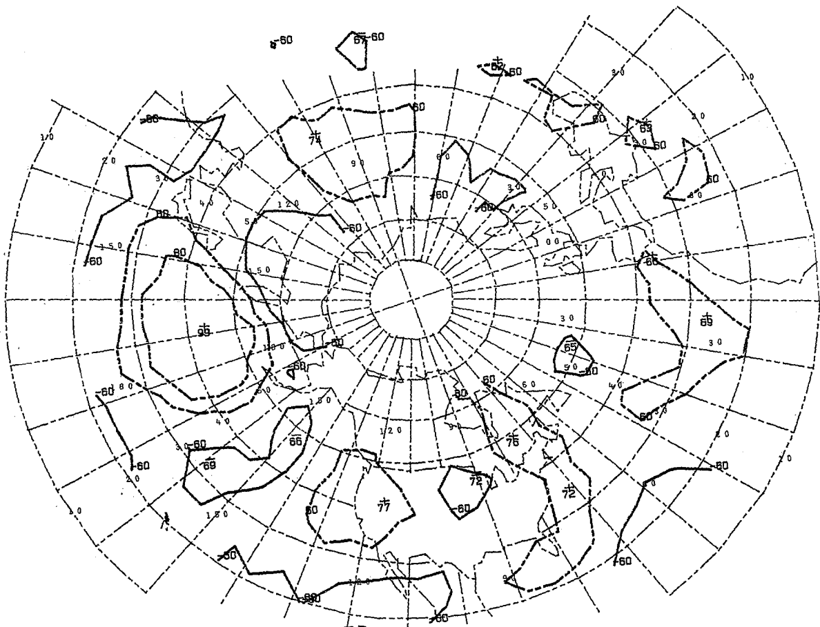
+ KEY AT170E 40N 18 CASES
