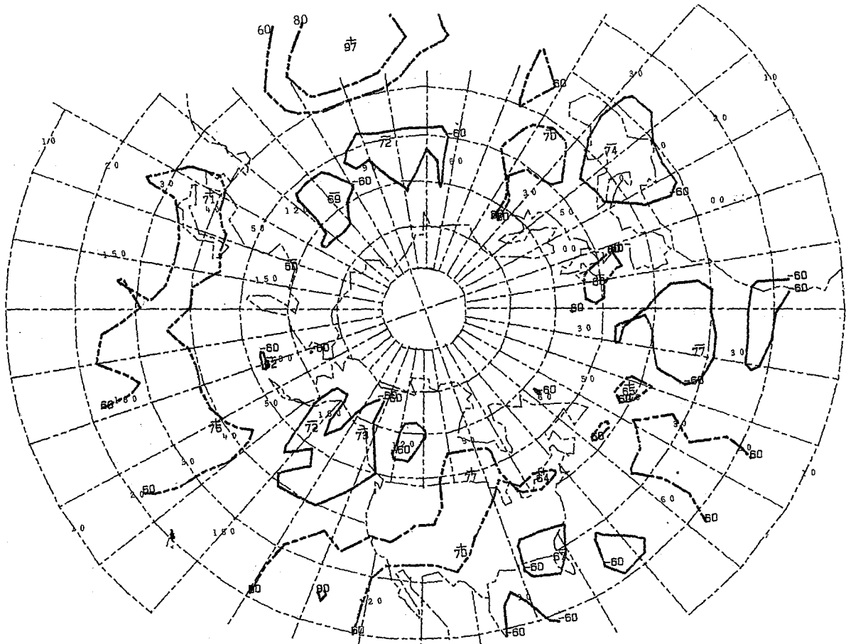
+ KEY AT 90E 30N 17 CASES
