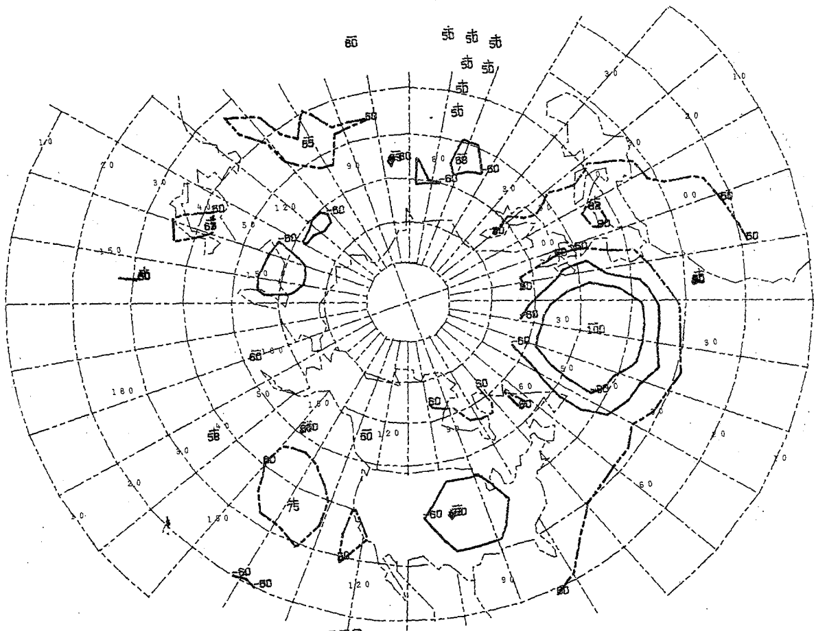
- KEY AT 30W 50N 22 CASES
