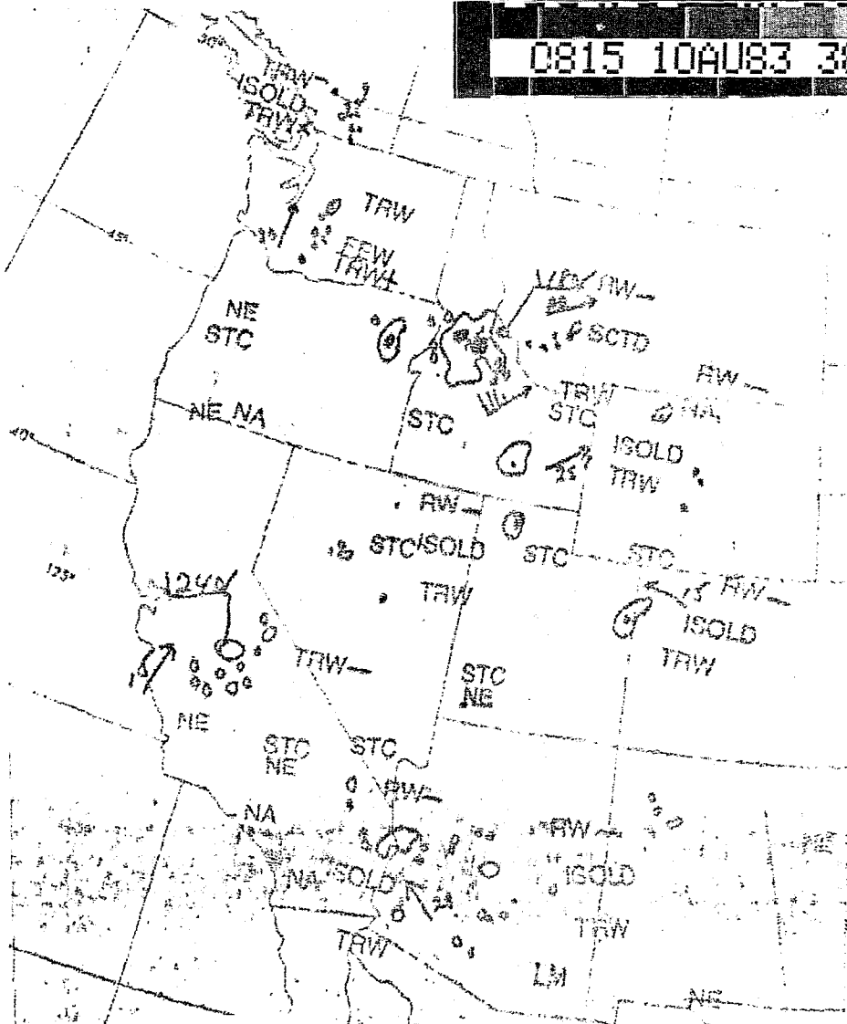
FIGURE 8. RADAR SUMMARY 0835Z August 10, 1983
