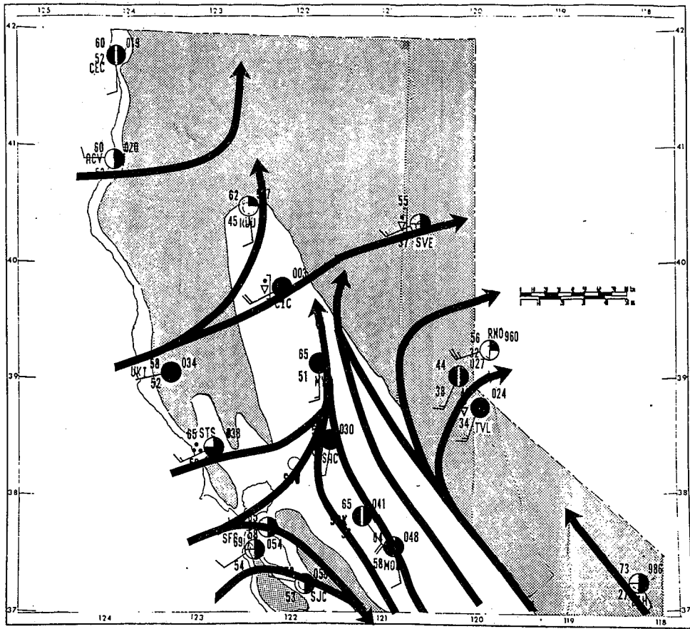
Figure 10c. As in Figure 8d, except for 2100 UTC (1300 LST).
