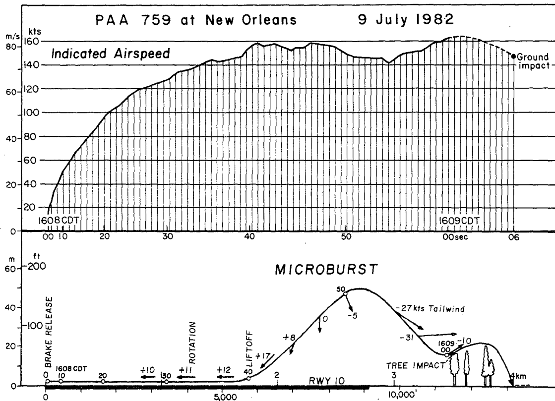
FIGURE 2 FLIGHT PATH AND INDICATED AIRSPEED OF PAA 759 AT THE NEW ORLEANS AIRPORT ON 9 JULY 1982. ACCORDING TO THE AUTHOR'S RECONSTRUCTION, THE AIRCRAFT REACHED 163 FT. (50 m) AGL. THEREAFTER, IT DESCENDED TO 52 FT. (16 m), CONTACTING A TREE ON THE EAST SIDE OF WILLIAMS BLVD. (FUJITA, 1985)
