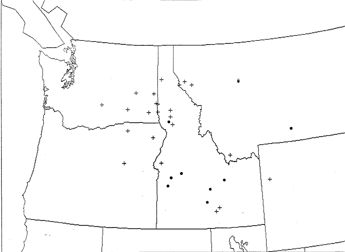
Fig. 1. Plot of all severe weather reports for the 24-hour period beginning at 1200 UTC 6 July 1995. Dark circles indicate hail reports while the cross symbol represents wind gusts or damage. Triangle represent tornadoes and diamond shapes indicate hail and wind damage reported at the same location.
