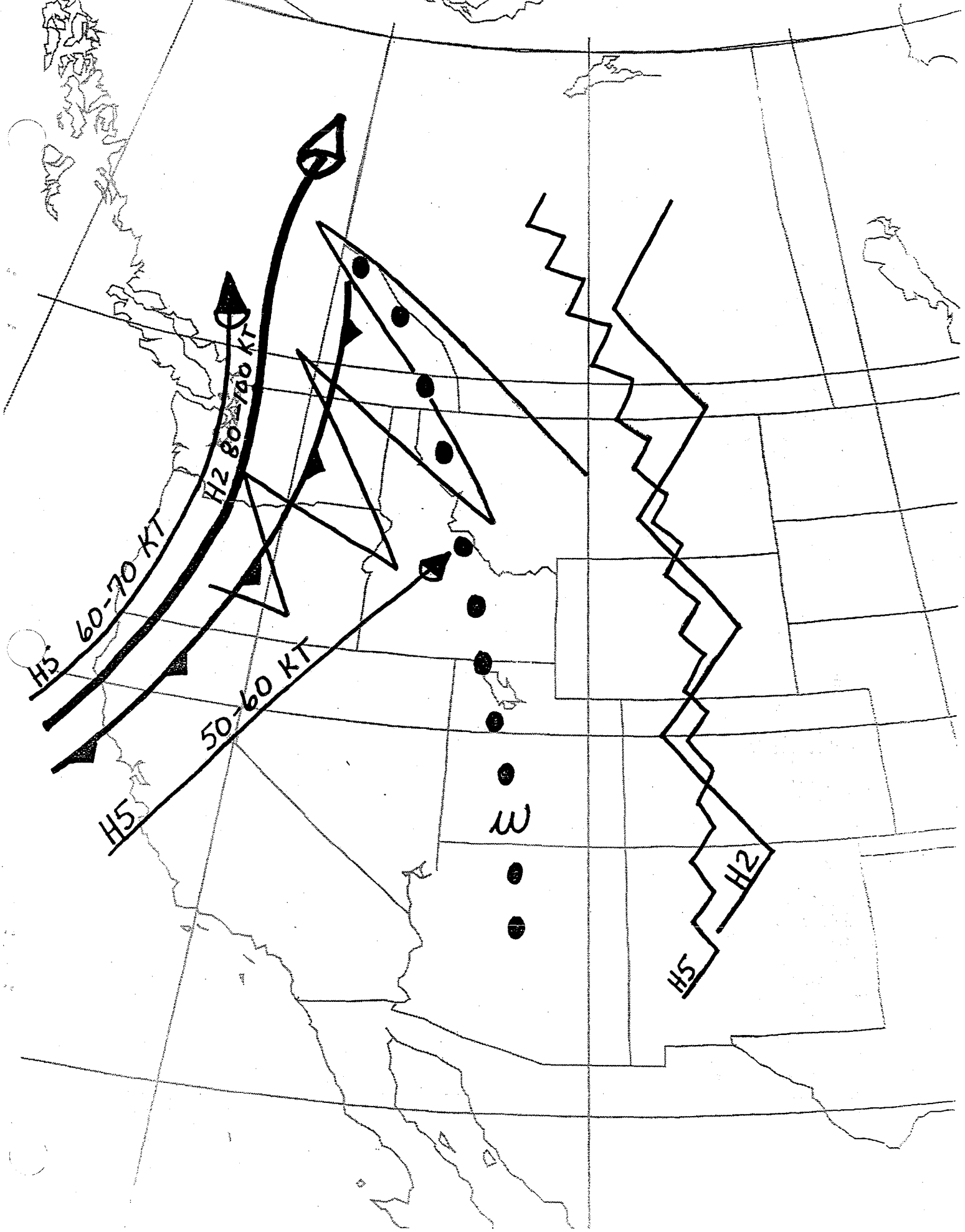
Fig. 13. Same as Fig. 4 but for 0000 UTC 10 July 1995.
