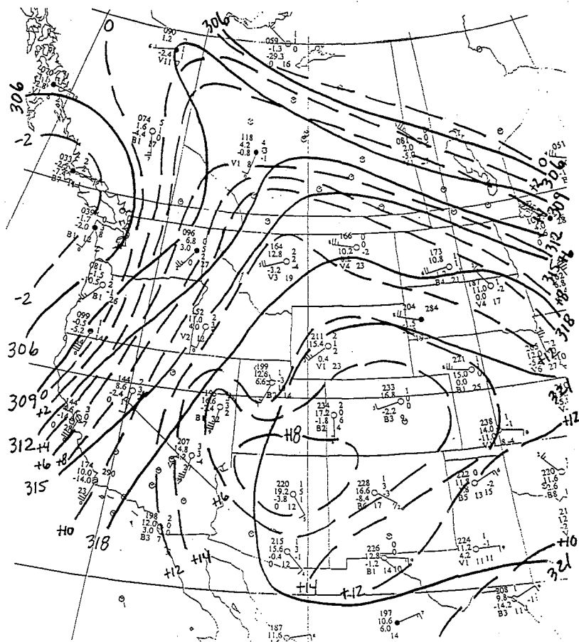
Fig. 12. Same as Fig. 5 but for 0000 UTC 10 July 1995.
