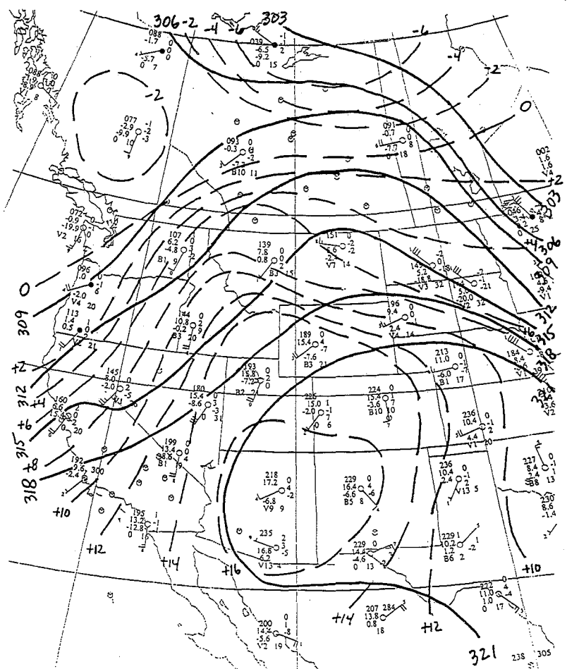
Fig. 7. Same as Fig. 5 but for 0000 UTC 7 July 1995.
