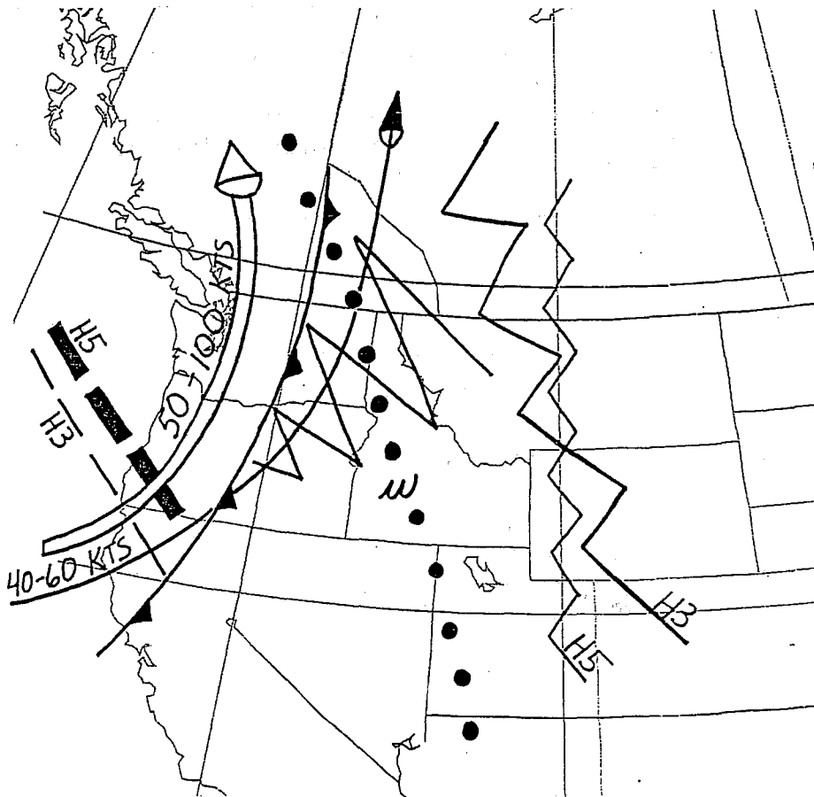
Fig. 4. Mean composite chart at 0000 UTC for Pattern A SSWEs affecting Washington and Oregon. Dotted line denotes 850 mb thermal ridge. Frontal boundary is position of 700 mb front. Long dashed lines labeled H5 and H3 indicate trough axis positions at 500 and 300 mb. Thin line with arrow indicates the jet axis at 500 mb while thick line with arrow represents the jet axis at 300 mb. Broad zigzag line shows an area of 500 and 300 mb diffluence while 500 and 300 mb ridge axes are denoted by long, north-south oriented narrow zigzag line.
