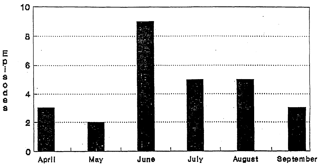
Fig. 3. Monthly distribution of SSWEs during the period from 1955 through 1993.
