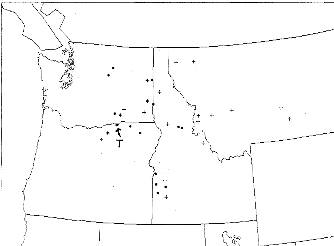
Fig. 2. Same as Fig. 1 but for the 24-hour period beginning at 1200 UTC 9 July 1995. Note the letter "T" indicates the location of a tornado.
