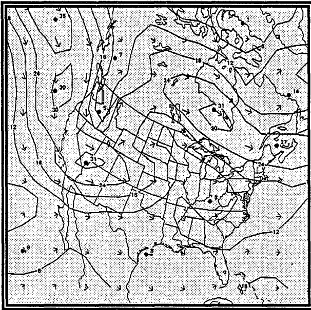
Fig. 3c: 250mb WINDS. A deep trough sets over the western states, and a jet maximum is located over southern Nevada. There is still difffluence aloft, enhancing the lift.
