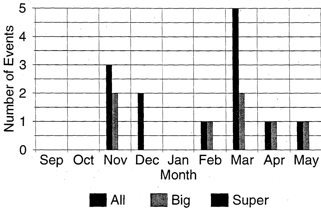
Figure 24c - Snowfall Distribution - West Flow
