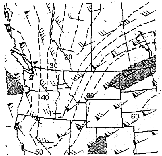
C) 250MB Wind (knots)
