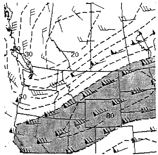
C) 250MB Wind (knots)
