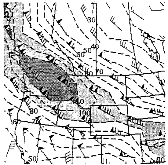
C) 250MB Winds (knots)
