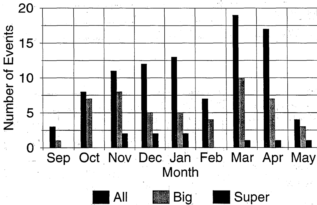
Figure 23 - Snowfall Distribution - All Flow Patterns
