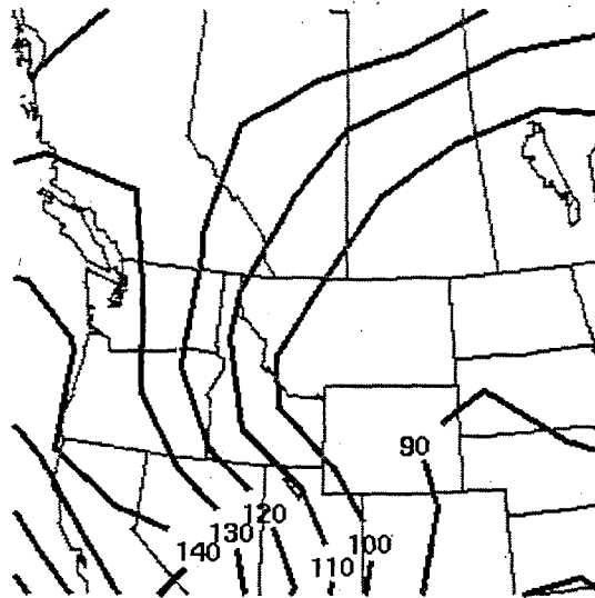
A) 500MB Heights (m)
