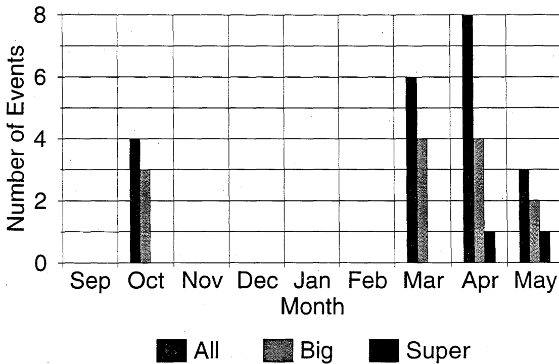
Figure 24e - Snowfall Distribution - Closed Low
