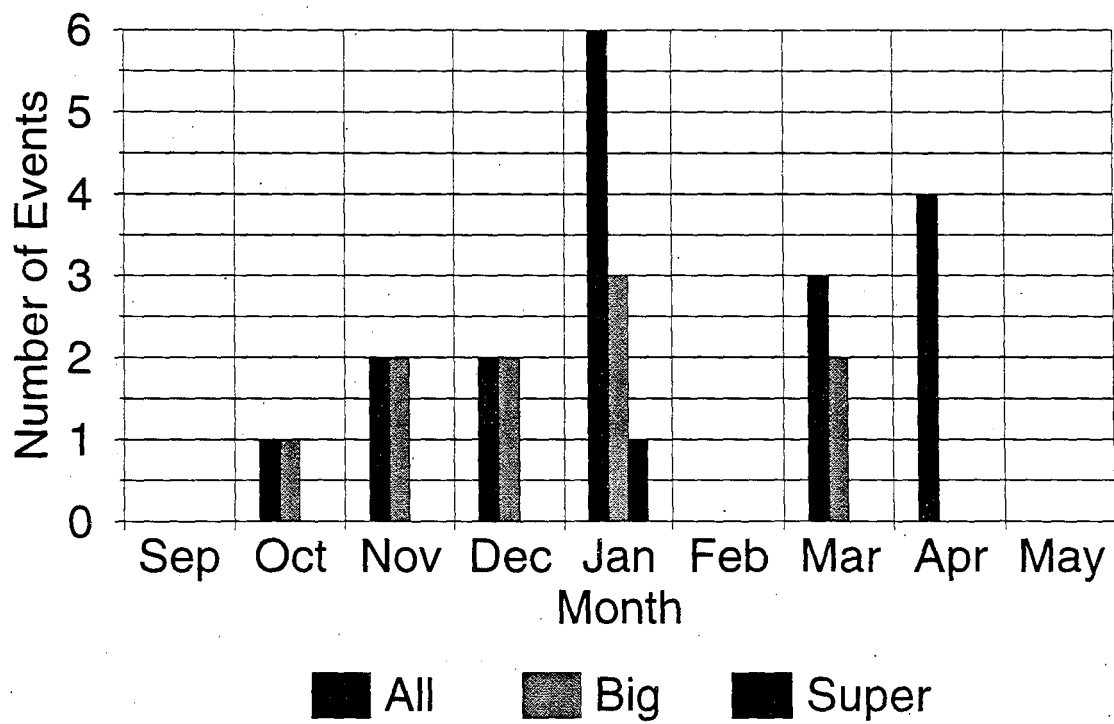
Figure 24a - Snowfall Distribution - Southwest Flow
