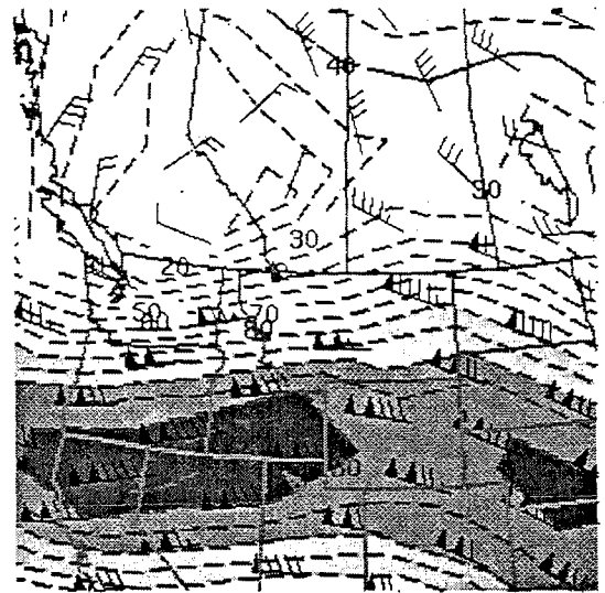
C) 250MB Winds (knots)
