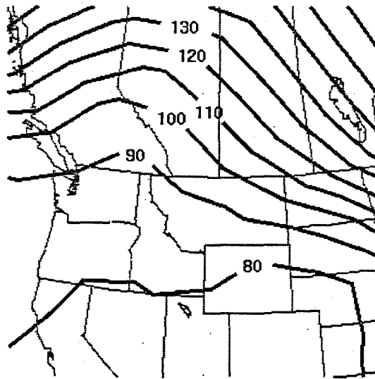
A) 500MB Heights (m)
