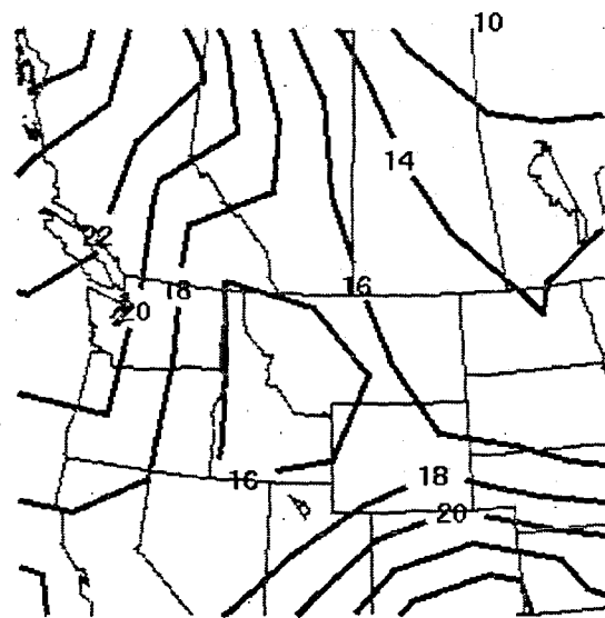
C) 250MB Winds (knots)
