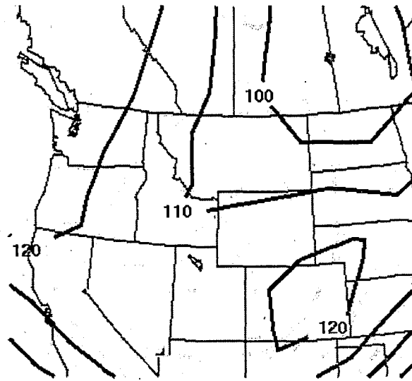
A) 500MB Heights (m)
