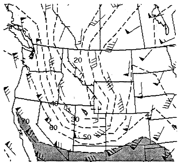
C) 250MB Winds (knots)
