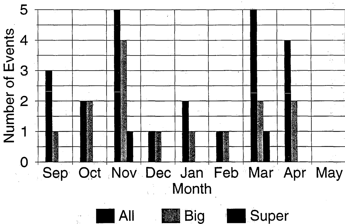
Figure 24b - Snowfall Distribution - Amplified Southwest Flow
