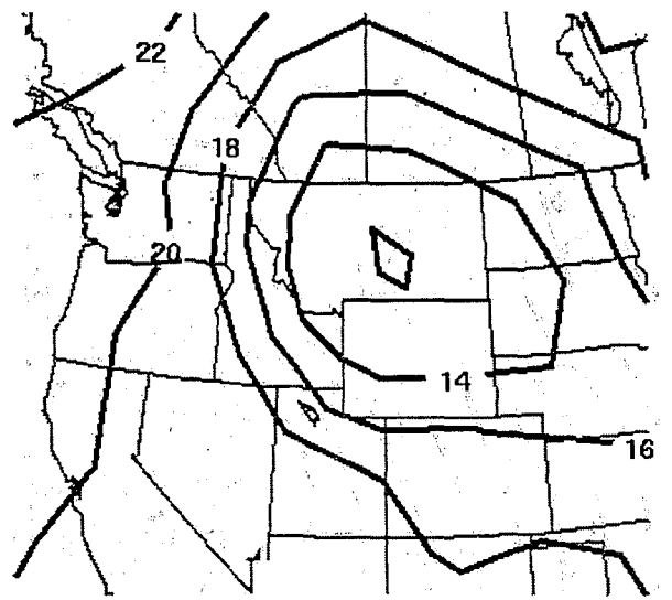
C) 250MB Winds (knots)
