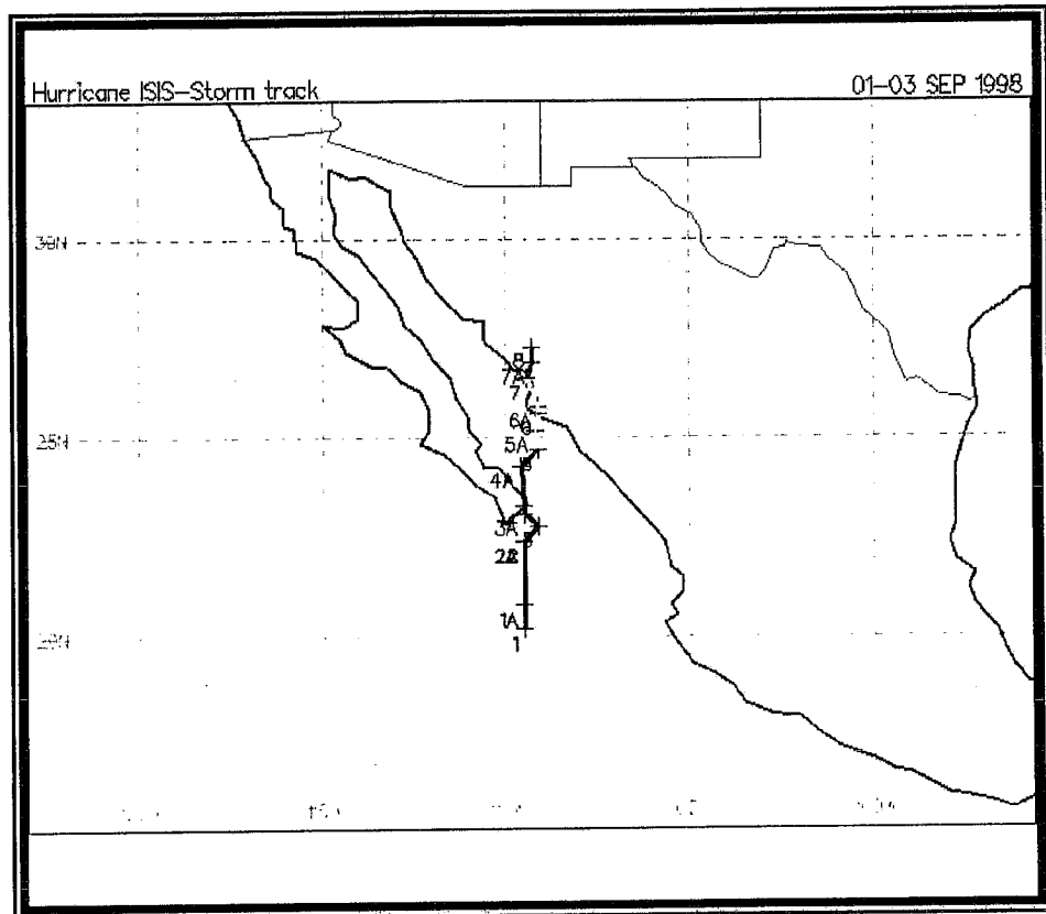
Figure 39 ..... T.S. (1-4) Sep. 01/21Z - 02/18Z; HUR. (5-6) Sep. 03/00Z - 06Z; T.S. (7-8) Sep. 03/12Z-15Z
