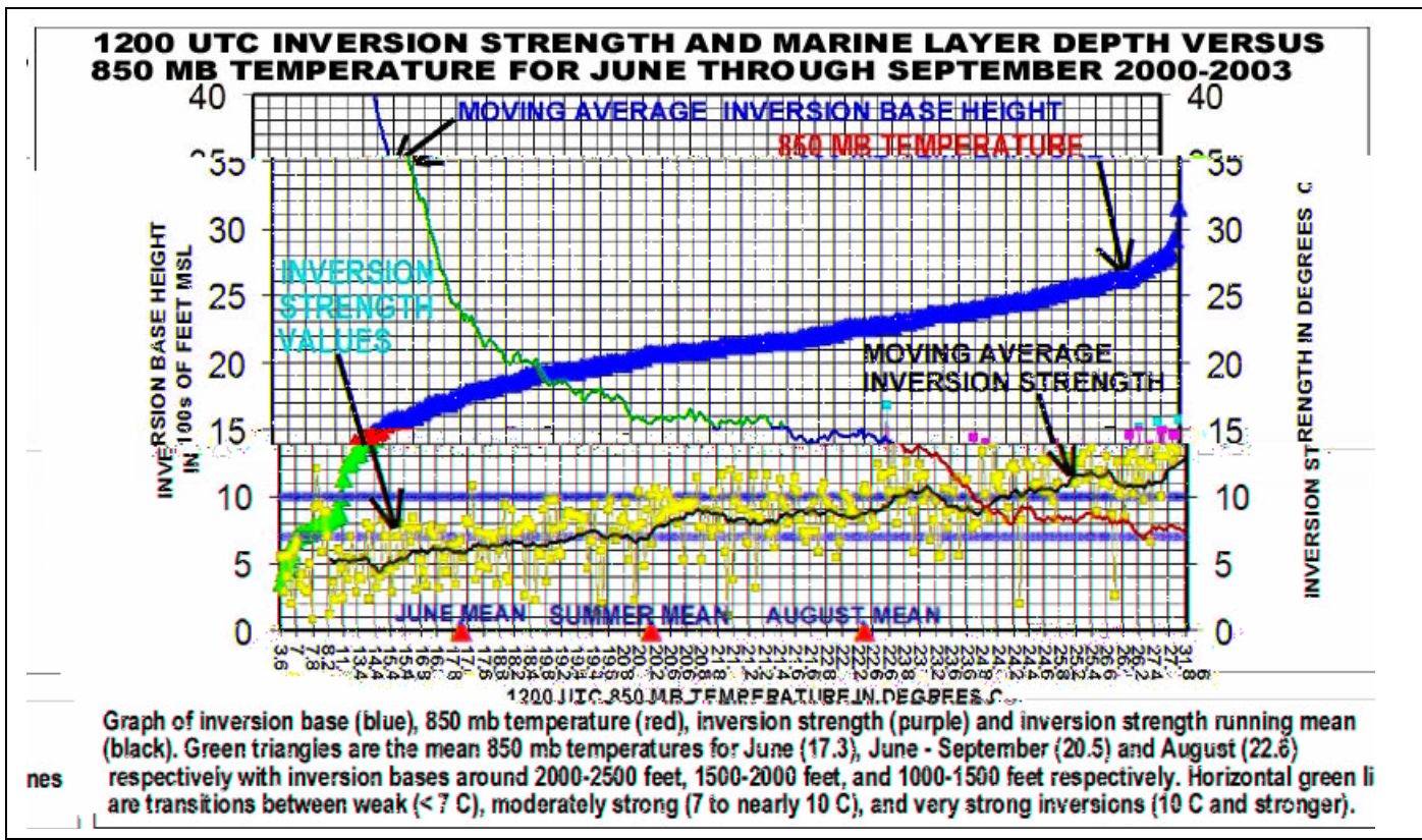
Fig. 5. Basically, the above graph shows how changes in the 850 mb temperature affects the inversion base height, inversion strength, and their relative values for June (deep marine layer), August (summer marine layer depth minimum) and the summer mean based on the 1200 UTC Miramar (KNKX) sounding. Lower 850 mb temperatures correlate well with deeper marine layers and weaker inversions. Higher 850 mb temperatures correlate well with shallower marine layers and stronger inversions. (The inversion usually weakens as the marine layer deepens, and strengthens as the marine layer becomes “more shallow”).
