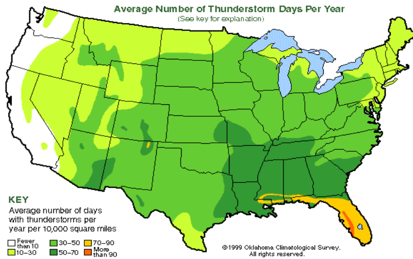
Figure 26. Average number of thunderstorm days (Oklahoma Climatological Survey)
