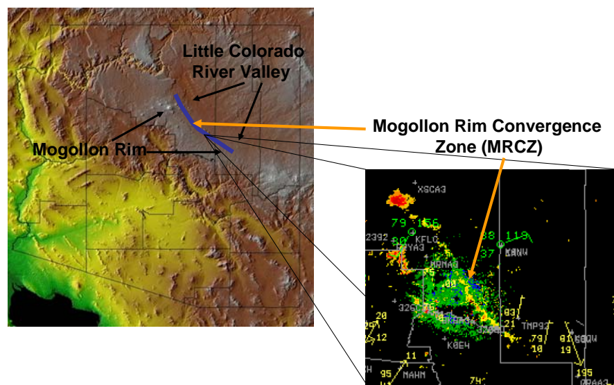
Figure 6. Mogollon Rim Convergence Zone (MRCZ) noted by Blanchard (2000)
