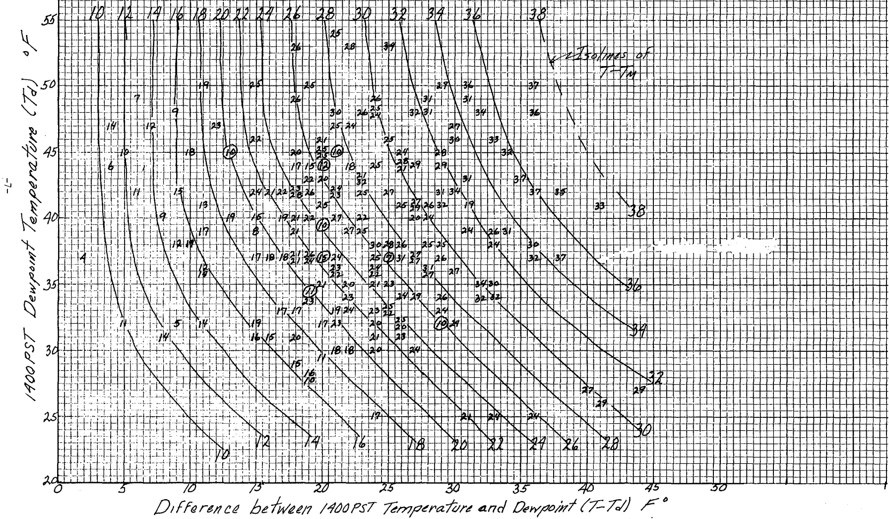
FIGURE 2. JOINT RELATIONSHIP OF 1400PST DEW POINT TEMPERATURE ( T_d ) AND DEW POINT SPREAD ( T-T_d ) WITH TEMPERATURE DROP FROM 1400PST TO MINIMUM ( T-T_m ) FOR MONTH OF APRIL AND CLOUDY CLASSIFICATION.
