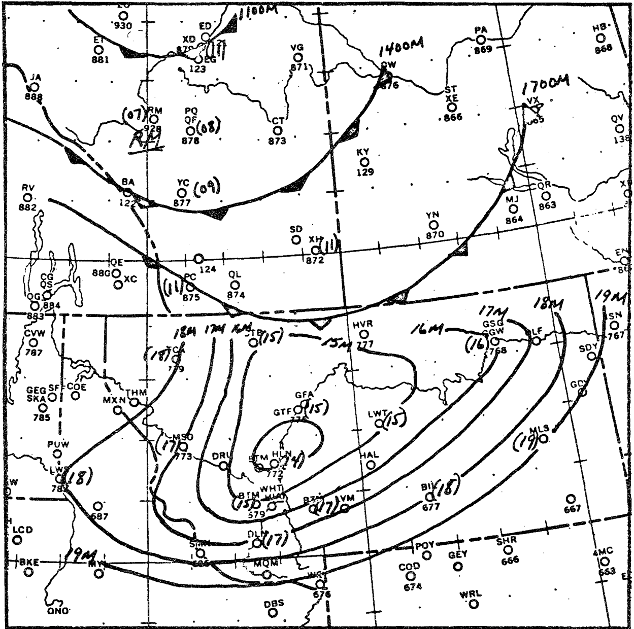
Figure 13. Positions of the advancing surface cold front in Alberta on December 11, 1963 and isochrones of time (MST) of beginning of snow in Montana. Time of snow onset at each station shown in parentheses.
