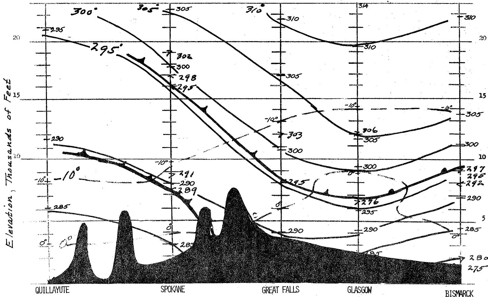
FIGURE 62. QUILLAYUTE-BISMARCK CROSS SECTION, 0000Z DECEMBER 3, 1967.
