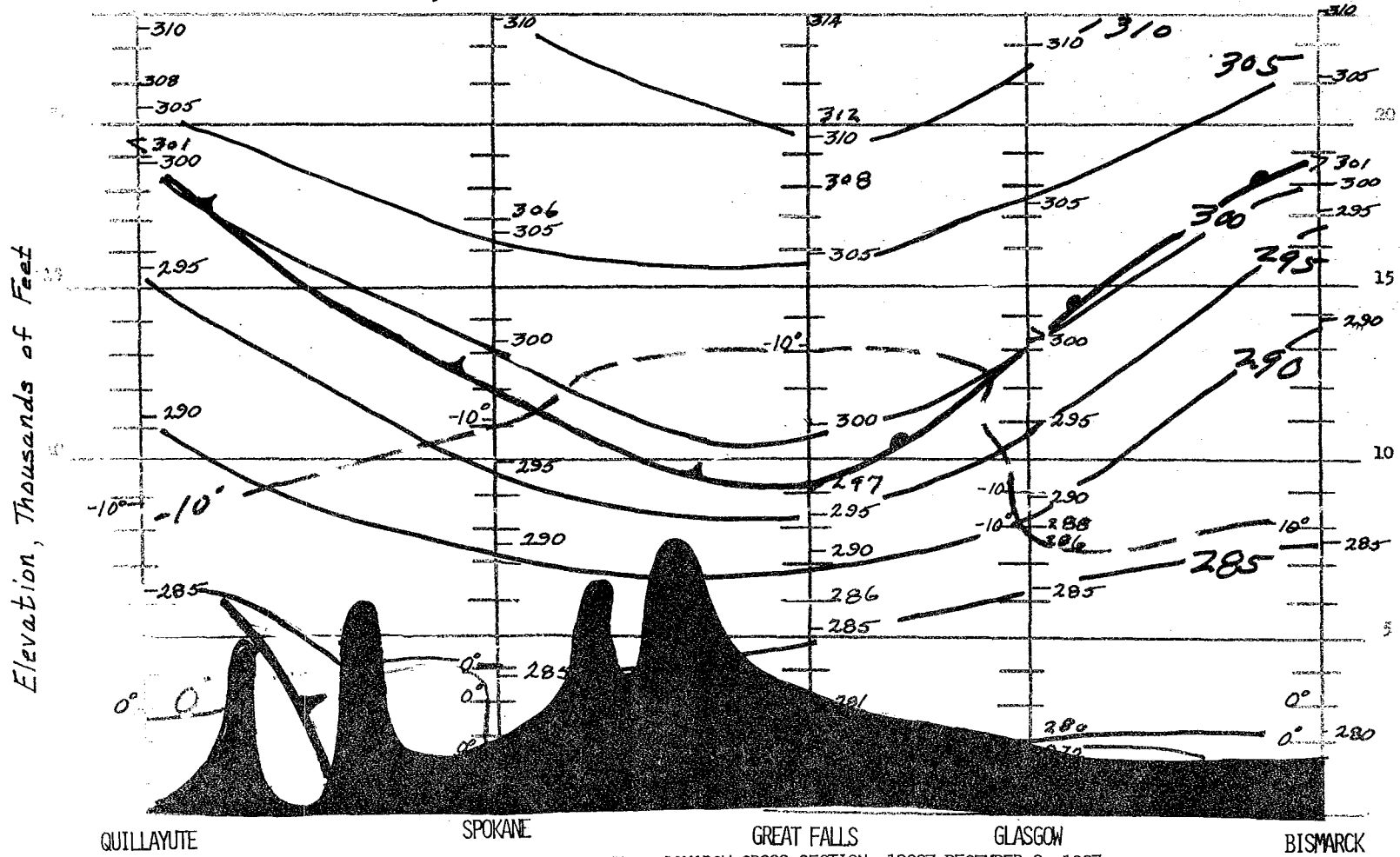
FIGURE 60. QUILLAYUTE-BISMARCK CROSS SECTION, 1200Z DECEMBER 2, 1967.
