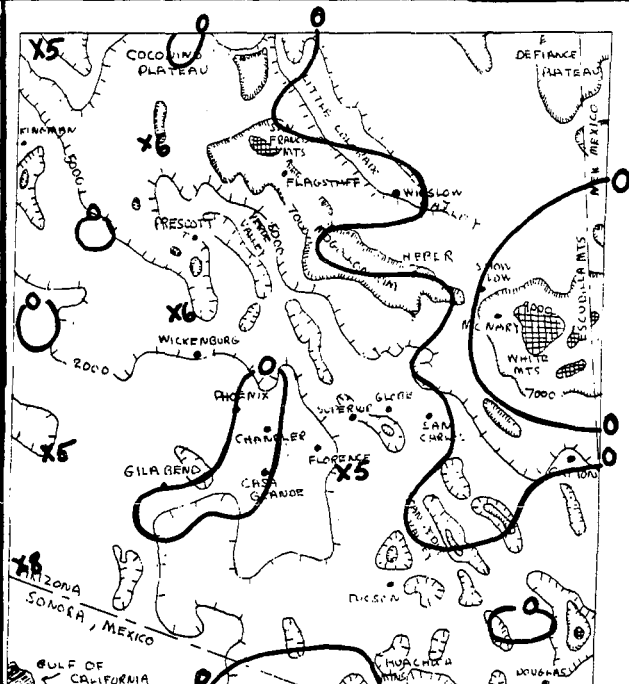
FIGURE 25. FREQUENCY OF RADAR ECHO DETECTION, 0830 MST, JULY-AUGUST 1971.
