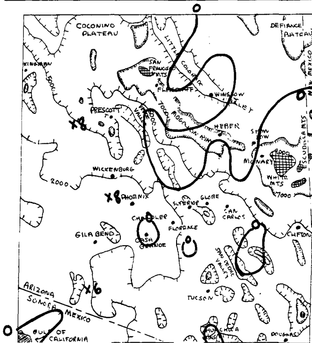
FIGURE 24. FREQUENCY OF RADAR ECHO DETECTION, 0730 MST, JULY-AUGUST 1971.
