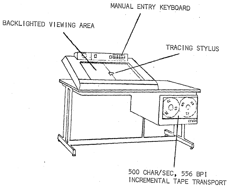
Figure 2. CALMA Model 302 Digitizer
