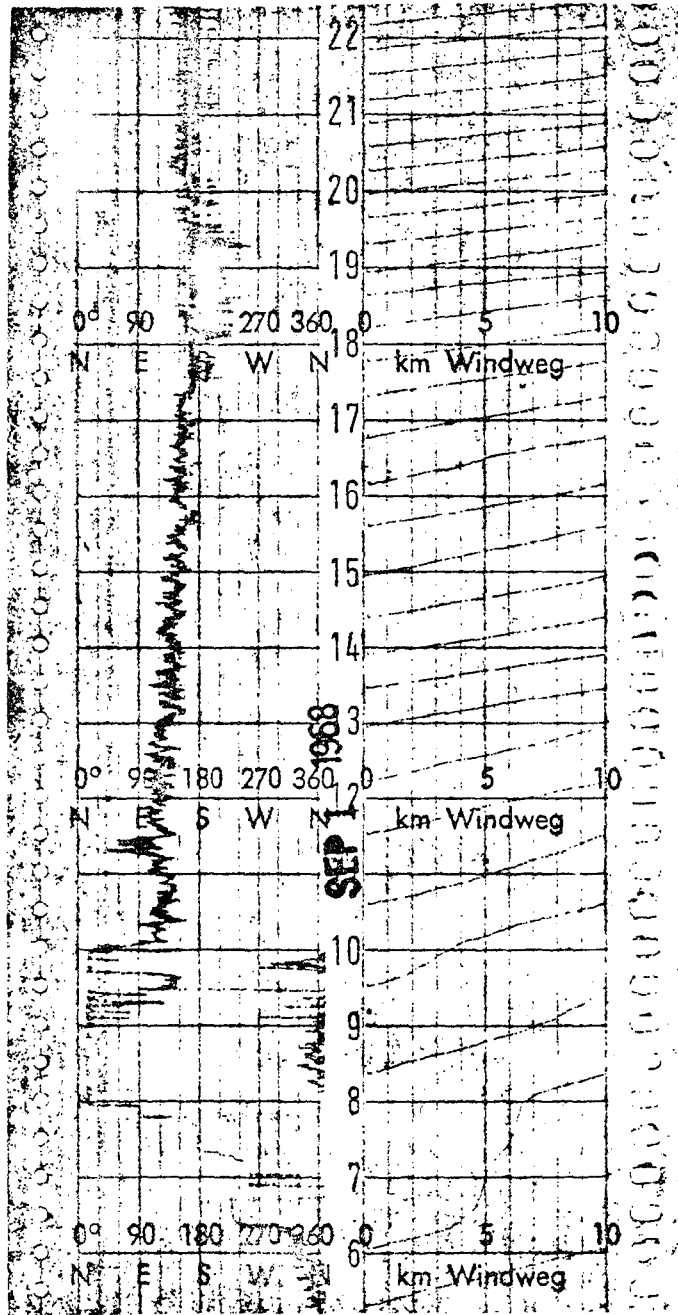
Figure 1. Portion of Wind Record from Epic Mechanical Wind Recorder
