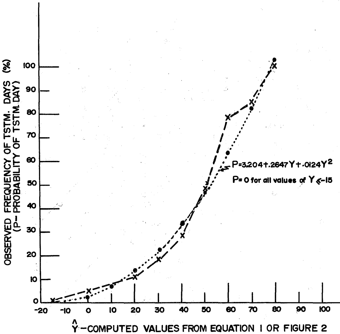
FIGURE 3. RELATIONSHIP BETWEEN COMPUTED VALUES OF \hat{Y} AND RELATIVE FREQUENCY OF THUNDERSTORM DAYS (CROSSES AND DASHED LINE) FOR AREA A. DOTTED CURVE REPRESENTS PARABOLA FITTED TO CROSSES.
