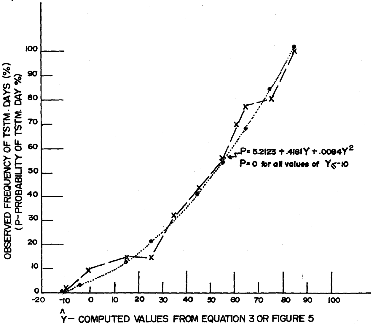
FIGURE 6. RELATIONSHIP BETWEEN COMPUTED VALUES OF \hat{Y} AND RELATIVE FREQUENCY OF THUNDERSTORM DAYS (CROSSES AND DASHED LINE) FOR AREA B. DOTTED CURVE REPRESENTS PARABOLA FITTED TO CROSSES.
