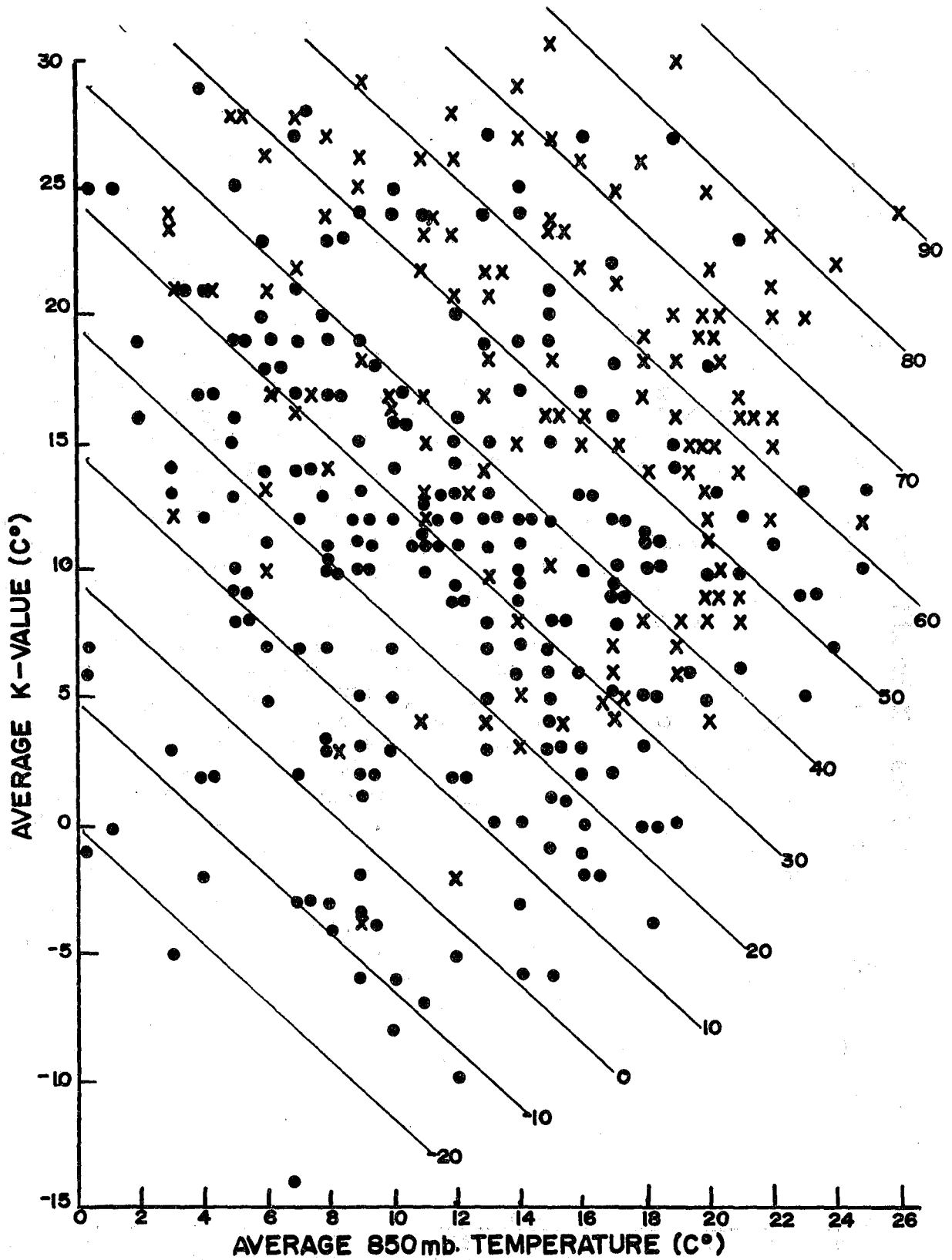
FIGURE 5. SCATTER DIAGRAM RELATING FREQUENCY OF THUNDERSTORM DAYS IN AREA B TO AVERAGE 850-MB TEMPERATURE AND AVERAGE K-VALUE COMPUTED FROM RADIOSONDE OBSERVATIONS AT BOISE, SALEM, QUILLAYUTE, AND SPOKANE. LINES REPRESENT SOLUTION OF LINEAR REGRESSION EQUATION: \hat{Y} = 2.36 X_1 + 2.04 X_2 - 19.91 . CROSS REPRESENTS THUNDERSTORM DAY; DOT NONTHTUNDERSTORM DAY.
