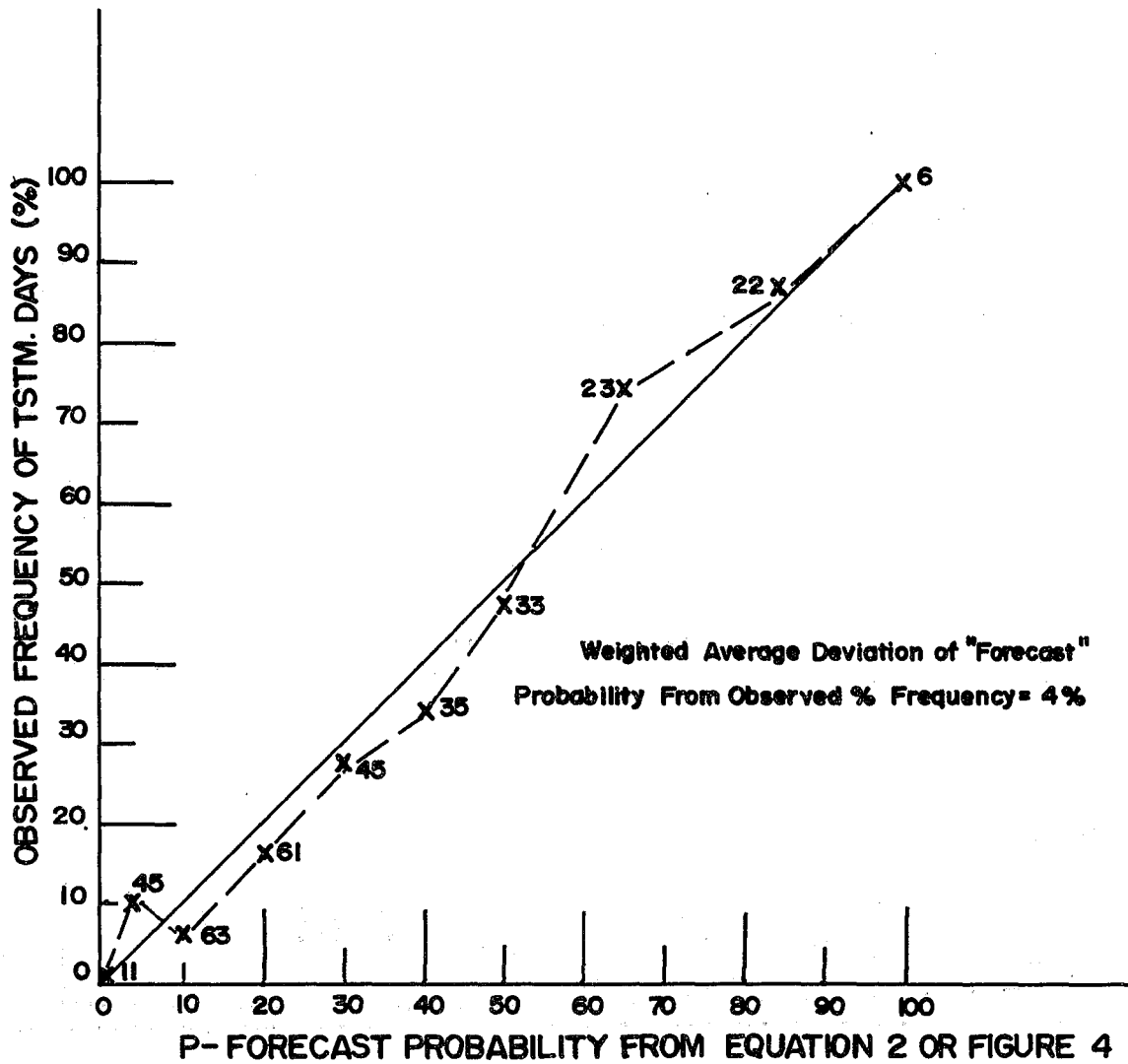
FIGURE 9. RELIABILITY GRAPH RELATING "FORECAST" PROBABILITIES FOR AREA A TO OBSERVED RELATIVE FREQUENCY OF OCCURRENCE OF THUNDERSTORM DAYS. NUMBER BESIDE EACH POINT IS NUMBER OF CASES IN FORECAST PROBABILITY CATEGORY (SEE TABLE 3).
