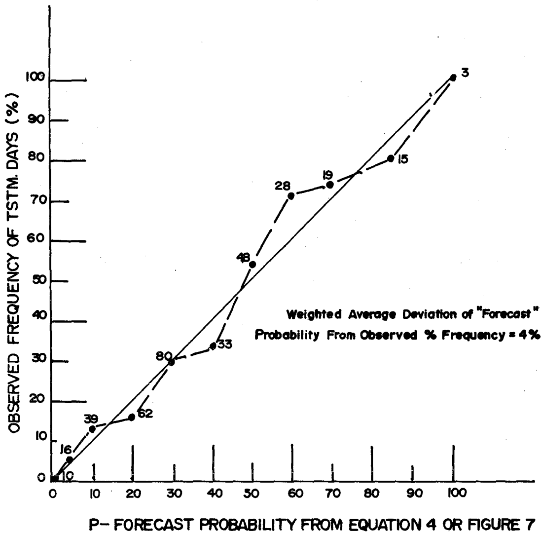
FIGURE 10. RELIABILITY GRAPH RELATING "FORECAST" PROBABILITIES FOR AREA B TO OBSERVED RELATIVE FREQUENCY OF OCCURRENCE OF THUNDERSTORM DAYS. NUMBER BESIDE EACH POINT IS NUMBER OF CASES IN FORECAST PROBABILITY CATEGORY (SEE TABLE 4).
