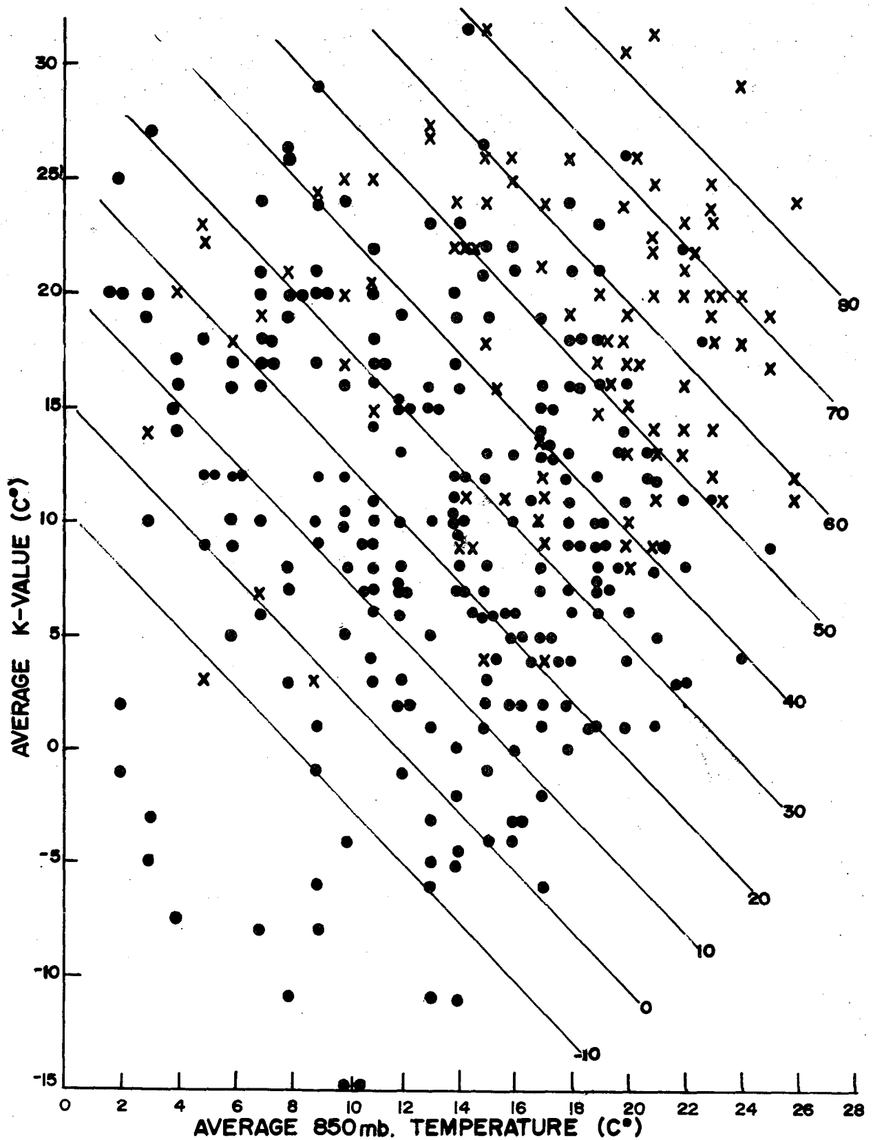
FIGURE 2. SCATTER DIAGRAM RELATING FREQUENCY OF THUNDERSTORM DAYS IN AREA A TO AVERAGE 850-MB TEMPERATURES AND AVERAGE K-VALUES COMPUTED FROM RADIOSONDE OBSERVATIONS AT BOISE, SALEM, MEDFORD, AND WINNEMUCCA. LINES REPRESENT SOLUTION OF LINEAR REGRESSION EQUATION: \hat{Y} = 2.59 X_1 + 1.99 X_2 - 30.90 . CROSS REPRESENTS THUNDERSTORM DAY; DOT NONTHUNDERSTORM DAY.
