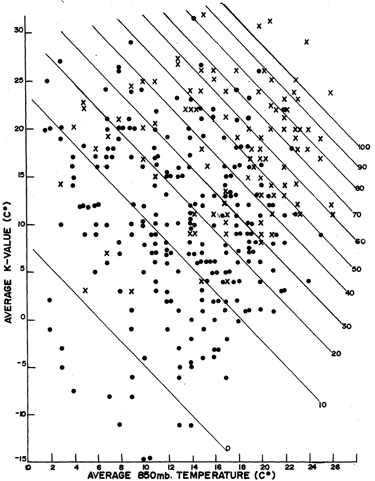
FIGURE 4. SAME AS FIGURE 2, EXCEPT LINES HAVE BEEN ADJUSTED TO REFLECT PARABOLIC RELATIONSHIP SHOWN IN FIGURE 3.
