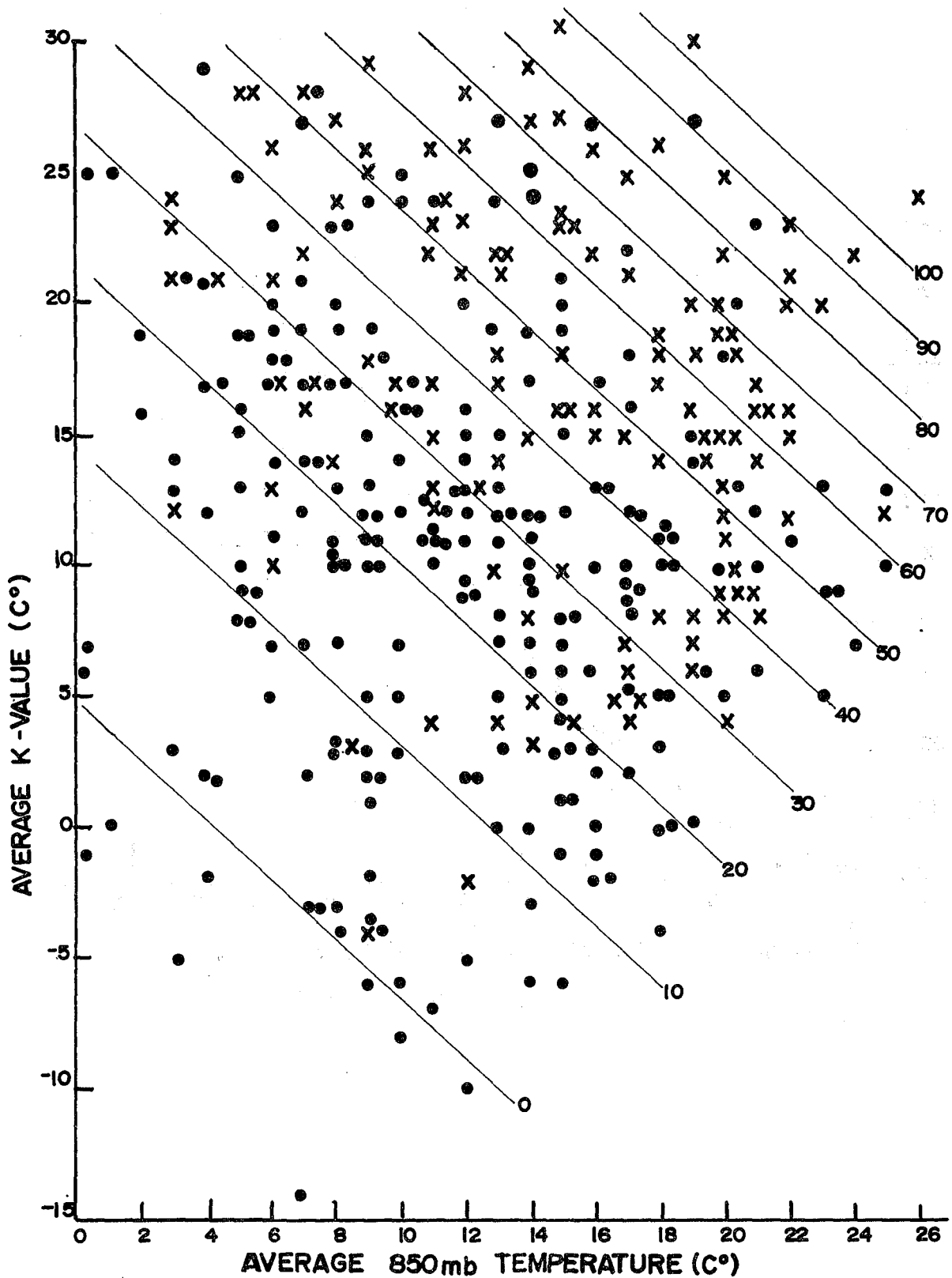
FIGURE 7. SAME AS FIGURE 5, EXCEPT LINES HAVE BEEN ADJUSTED TO REFLECT PARABOLIC RELATIONSHIP SHOWN IN FIGURE 6.
