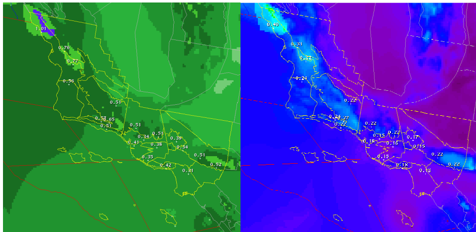
Figure 3 - The left image shows a gridded QPF forecast from the National Weather Service, Los Angeles/Oxnard Office. The image to the right is a gridded PRR forecast derived from the left image using an equation similar to equation 2.
