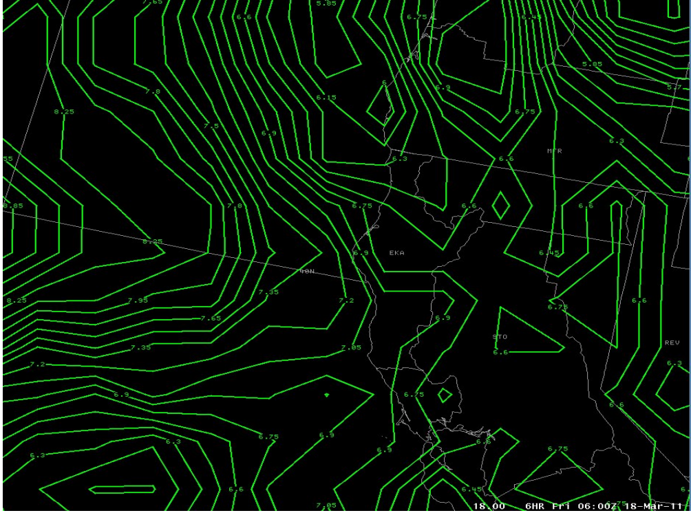
Figure 5: 925 to 850 MB lapse rates of 6 to 8 degrees C/km showing general instability.
