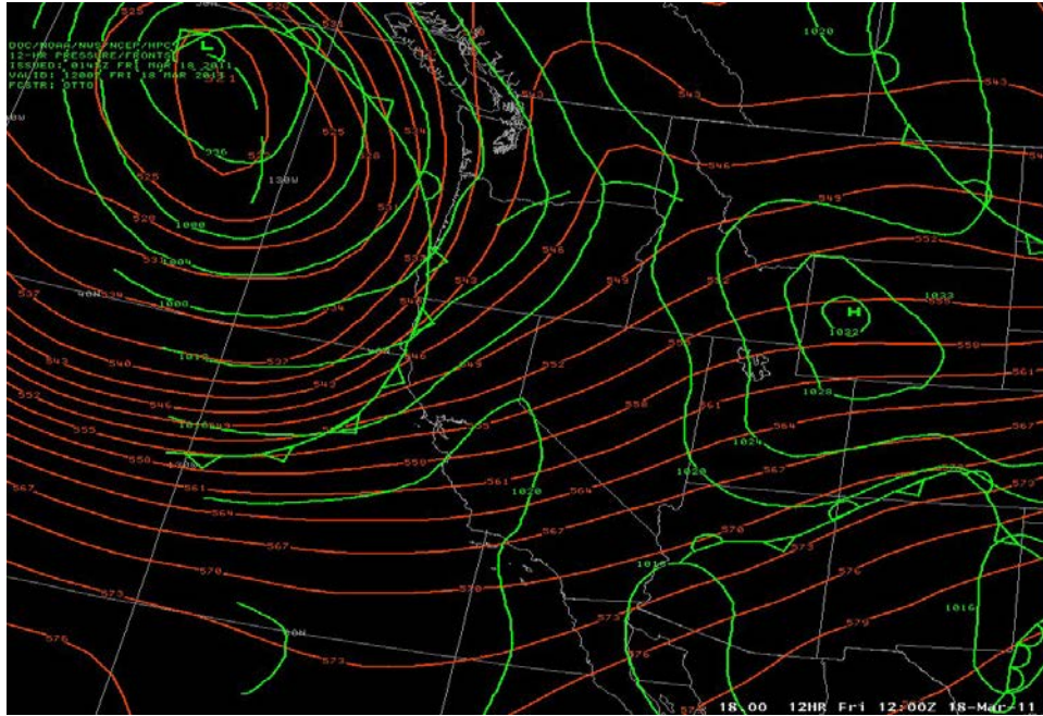
Figure 1: 500 MB heights with an overlaid NCEP surface analysis showing the typical set up of the cold front synoptic weather pattern over the eastern Pacific.
