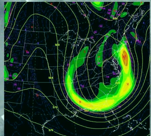
0000 UTC 27 December 2010
