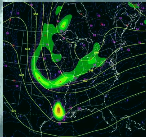
1200 UTC 25 December 2010
