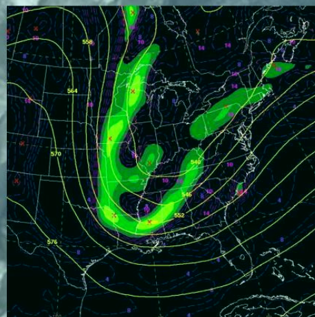
0000 UTC 26 December 2010
