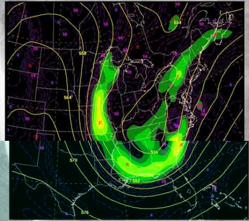
1200 UTC 26 December 2010
