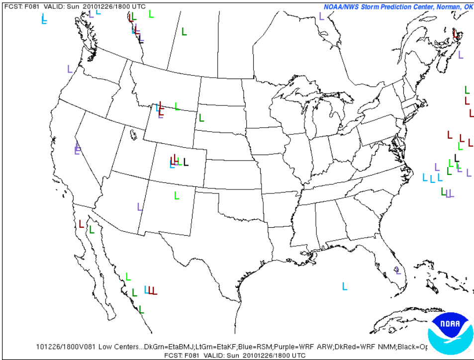
Fig. 38 SREF 81-hour SLP low center spaghetti forecast valid 18 UTC 26 December 2010.
