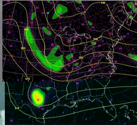
0000 UTC 25 December 2010
