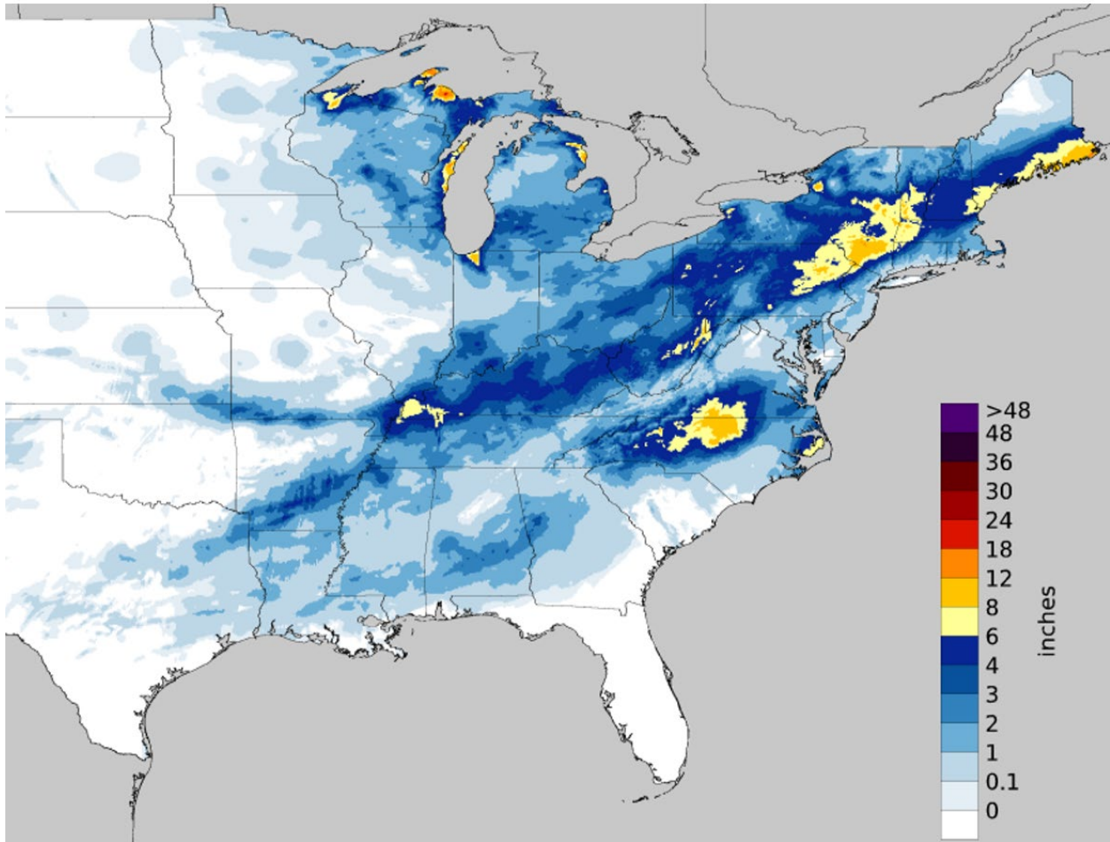
Figure 1: 72-hour observed snowfall analysis ending at 12 UTC January 18, 2018.
