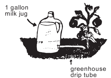
Figure 20.11. Trickle system for favorite plants (i.e., giant pumpkin, early tomatoes, etc.).
