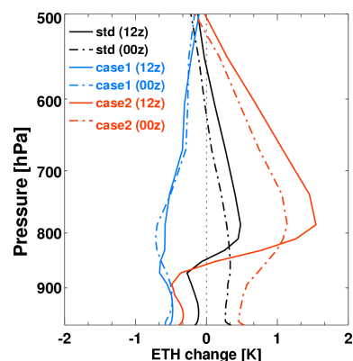
Fig. 10. Dust impact on the equivalent potential temperature (ETH) profiles at 00:00 UTC and 12:00 UTC averaged over the WAM region ( 6^{\circ} N– 17^{\circ} N and 15^{\circ} W– 10^{\circ} E) from WRF-Chem simulations in three cases with different dust absorption properties: std ( n_i = 0.003 ), case1 ( n_i = 0.0004 ), and case2 ( n_i = 0.006 ), where “ n_i ” represents the imaginary part of the refractive index of dust.
