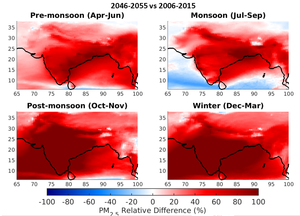
Figure S14. Seasonal distribution of the relative difference in surface PM 2.5 between the reference scenario and the FCE2050 scenario. The relative differences are calculated as: ([FCE2050 - \text{reference}] / \text{reference}) \times 100\% .
