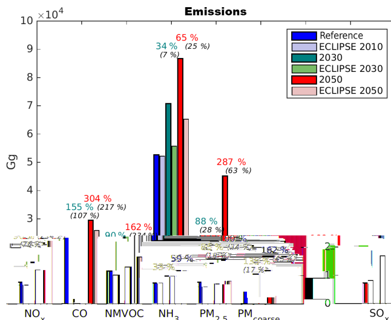
Figure 1. Annual emissions (in Gg \text{ yr}^{-1} ) used for the reference (2010), FC2030 and FC2050 scenarios (dark blue), and for 2030 (dark green) and 2050 (dark red), used for the FCE2030 and the FCE2050 scenarios over India, respectively. The variation of each compound with respect to the reference scenario is also provided by coloured percentage figure. The ECLIPSE emissions are also plotted for comparison and represented by light coloured bars. The variation of each compound with respect to ECLIPSE2010 scenario is also provided by italic black percentage figure given in parentheses.
