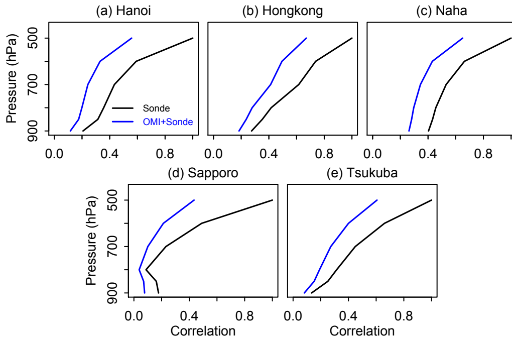
Figure S4. Correlation of OMI 850-400 hPa ozone and the boundary layer ozone assuming that the OMI were sensitive only to the free troposphere at \sim 500 hPa (where its sensitivity is maximum, Figure 3c) and not to the boundary layer. The black line is the correlation of ozone at different pressure levels with 500 hPa ozone in the sonde observations. The blue line is the estimated correlation of OMI 850-400 hPa with ozone at different layers if the satellite can only detect the signal at 500 hPa but not from other layers, as calculated using Equation 2. See text for more details.
