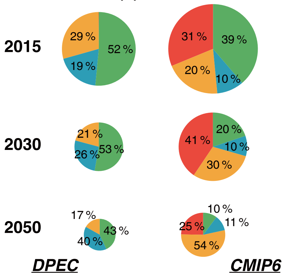
(c) BC
