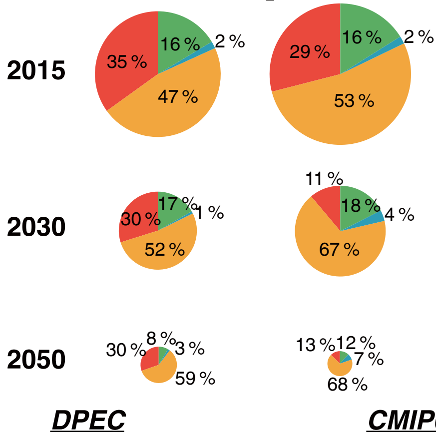
(a) SO 2
