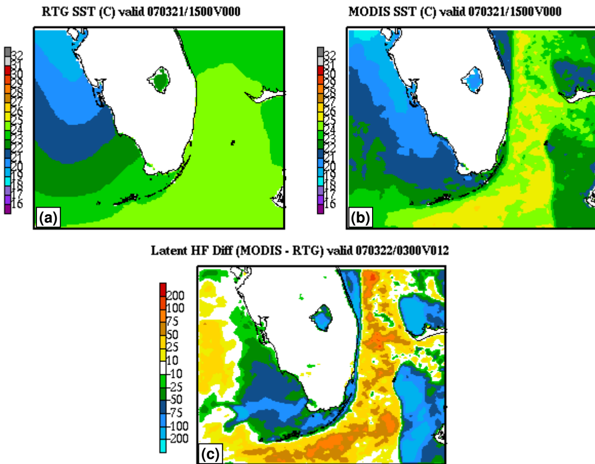
Figure 2. SSTs in the WRF simulation initialized at 1500 UTC 21 March 2007 for (a) the 1/12° RTG SST product, and (b) the MODIS composite. (c) Difference in 12-hour forecast latent heat flux ( \text{W m}^{-2} ) between the MODIS and RTG WRF simulations, valid at 0300 UTC 22 March 2007.
