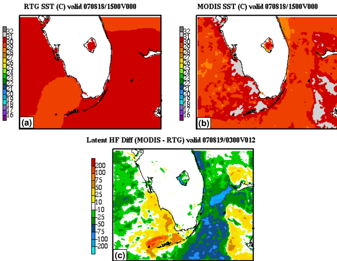
Figure 3. Same as in Figure 2, except showing the forecast initialized at 1500 UTC 18 August 2007.
