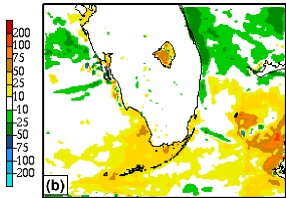
Figure 8. WRF simulated latent heat flux differences (MODIS – RTG) valid at 0900 UTC 15 June for the (a) 18-h forecast initialized at 1500 UTC 14 June, and (b) 12-h forecast initialized at 2100 UTC 14 June.
