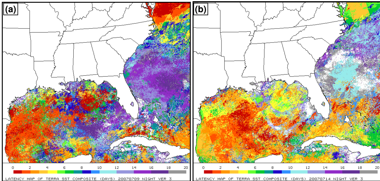
Figure 7. Latency of MODIS SST composite in days, according to the scale provided, valid for the 0400 UTC composite on (a) 9 July, and (b) 14 July. Notice the dramatically improved latency values around the Florida Keys by 14 July in (b).
