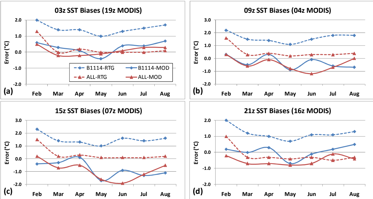
Figure 5. Same as Figure 4 except for the bias scores.
