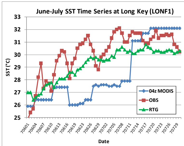
Figure 6. June–July 2007 time series of daily 0900 UTC observed SSTs at Long Key, FL (LONF1), daily RTG-initialized SSTs, and MODIS-initialized SSTs interpolated to station LONF1 from the 0400 UTC composite, according to the legend provided.
