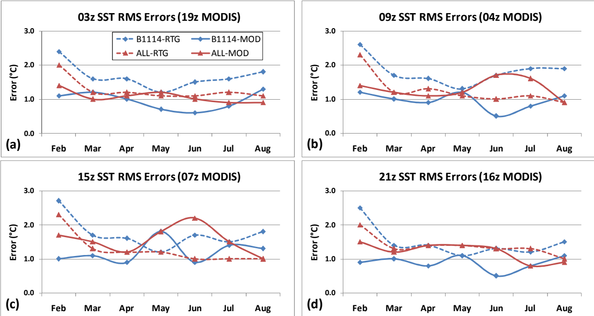
Figure 4. Monthly sea surface temperature root mean square errors for all 6 marine stations labeled in Figure 1, and buoy B1114 on the Florida east coast at model initialization times (a) 0300 UTC, (b) 0900 UTC, (c) 1500 UTC, and (d) 2100 UTC.
