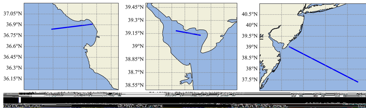
Figure 1. Geographical locations of the selected RSP legs.
