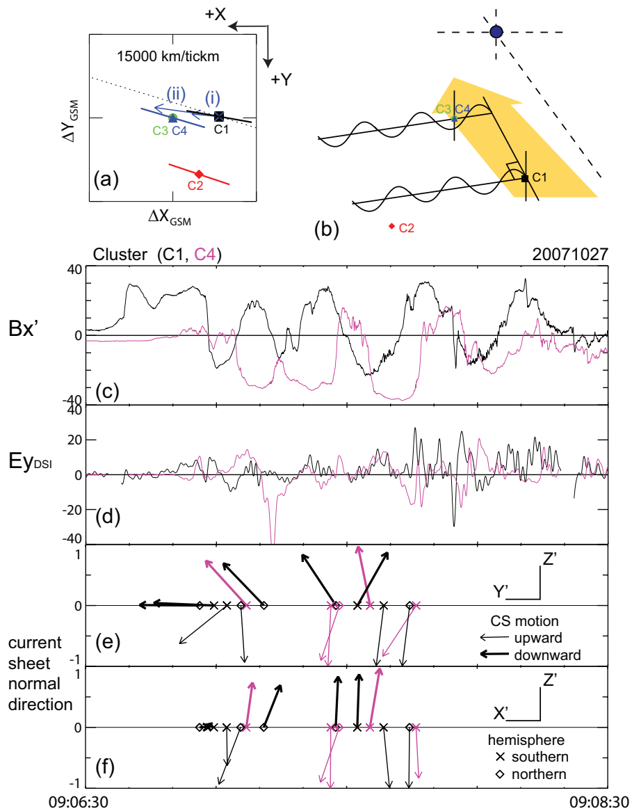
Fig. 5. (a) CODIF proton flow vector at (i) 09:06:53 and (ii) 09:07:01 UT and the maximum variance direction for the four spacecraft. The dotted line shows the X' axis direction. (b) Schematic drawing showing the relationship between the fast flows and current sheet oscillation. (c) B_{X'} and (d) 1s averaged E_Y from C1 and C4 between 09:06:30 and 09:08:30 UT. Normal direction of the current sheet for each half-hemisphere crossings projected on the (e) Y' - Z' plane and the (f) X' - Z' plane.
