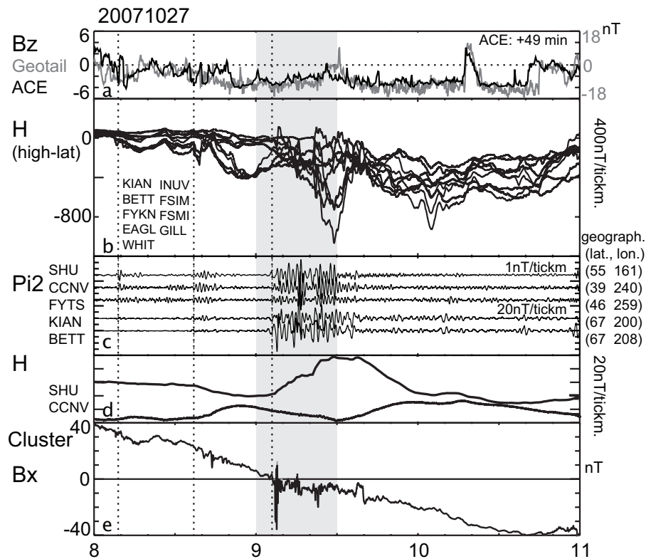
Fig. 1. (a) IMF B_Z from ACE and B_Z component from Geotail in the magnetosheath at (X, Y, Z) = (-2, 16, 13) R_E , (b) H component of the high-latitude magnetograms from north-American stations, (c) mid-latitude and high-latitude Pi2 (filtered H component between 40 and 150 s), (d) positive bay, and (e) B_X component of C3. The three positive bay onsets discussed in the text are shown by the vertical line. The gray hatched time shows the third substorm event when Cluster crossed the center of the current sheet.
