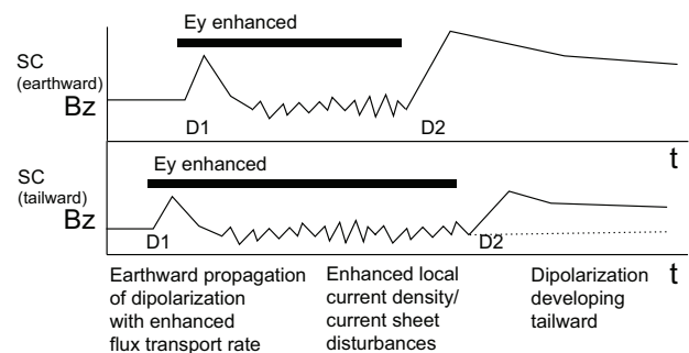
Fig. 8. Schematic representation of virtual spacecraft observations separated in X (fast flow direction) describing the two different types of dipolarization.
