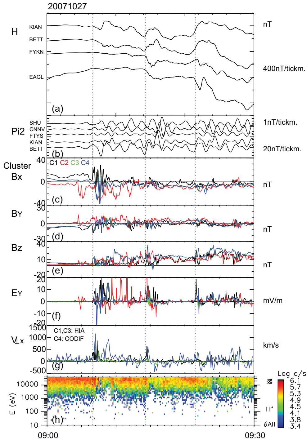
Fig. 3. (a) H -component from selected high-latitude stations, (b) Pi2 , (c–e) three components of the magnetic field and (f) E_y from the four Cluster, and (g) X component of the perpendicular plasma flow relative to the magnetic field from C1, C3, and C4, and (h) energy spectra for proton from C4. The three vertical line denotes the onset time of dipolarization at C1, i.e., 09:06:40, 09:14:20, 09:21:30 UT.
