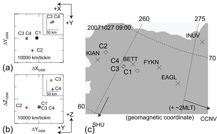
Fig. 2. Relative position of Cluster in (a) X - Y , (b) Y - Z plane, and (c) location of the foot-points of Cluster.
