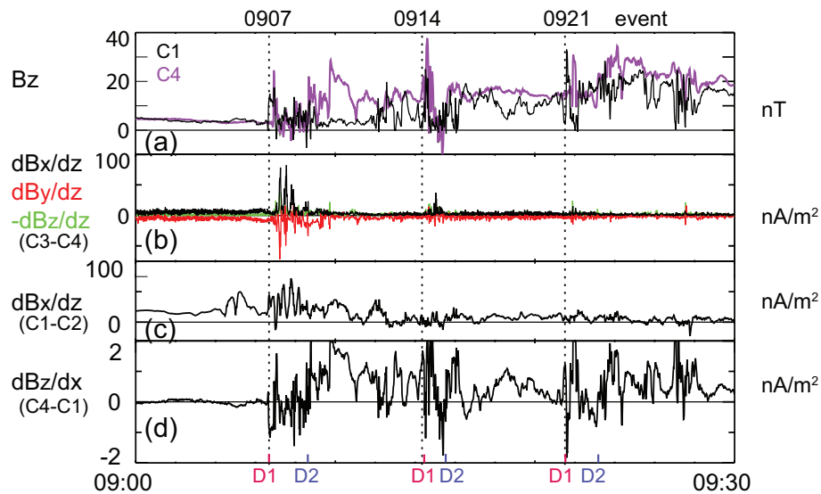
Fig. 6. Characteristics of the current sheet between 09:00 and 09:30 UT. (a) B_z from C1 and C4, (b) magnetic field gradient obtained from C3 and C4 assuming that the main gradient direction is across the current sheet, i.e., Z , (c) \Delta B_x/\Delta z using C1 and C2, and (d) \Delta B_z/\Delta x using C1 and C4.
