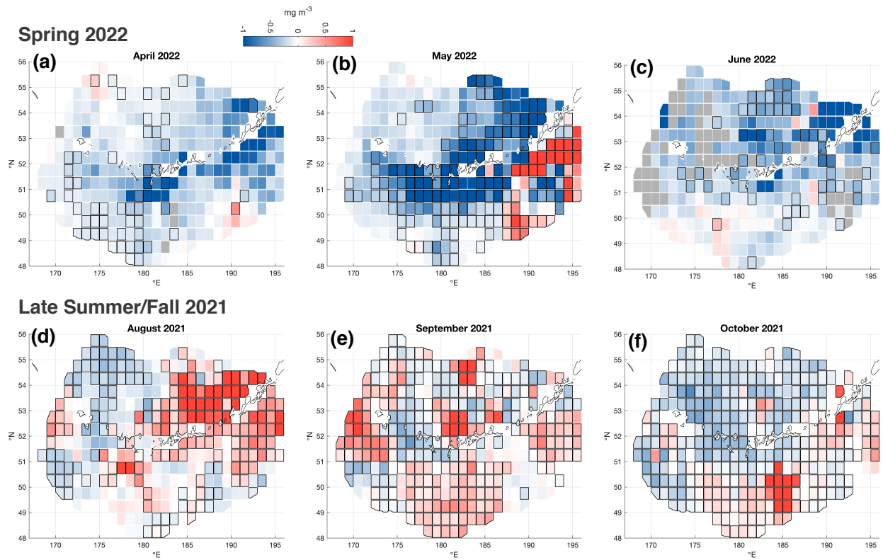
Figure 23: Spatial patterns in monthly-average anomalies from the seasonal cycle, April–June 2022 (top row) and August–October 2021 (bottom row). Anomalies are composed from data averaged with Alaska Department of Fish and Game Statistical Areas, restricted to areas of size >2500 square kilometers. Areas with a black boundary have a monthly anomaly exceeding the 95% confidence bounds. Gray shading indicates areas not sampled within a given month.
