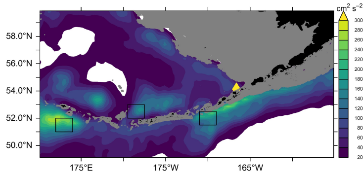
Figure 20: Eddy Kinetic Energy computed from satellite sea surface height (SSH) averaged over January 1st, 1993 – December 31st, 2021. Squares denote regions over which EKE was averaged for Figure 21.
