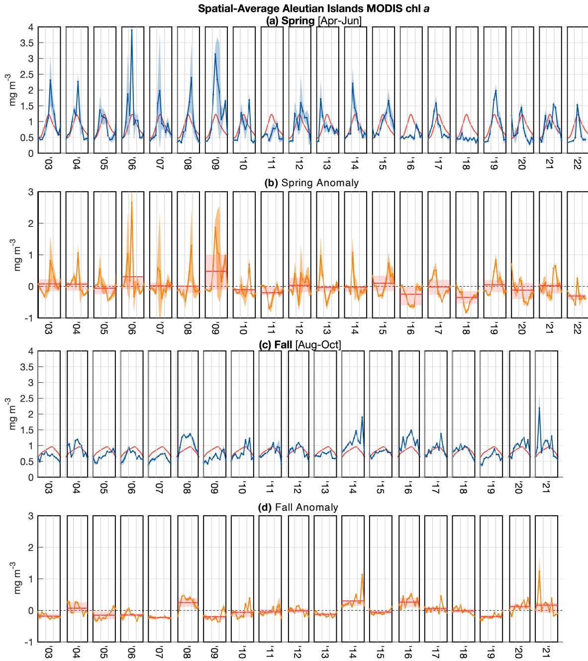
Figure 22: Time series of spatial-average Aleutian Islands chlorophyll a in MODIS 8-day composites, for the months of (a)-(b) April to June, and (c)-(d) August to October. Panels (a) and (c) show the full time series, while (b) and (d) show anomalies from a composite seasonal cycle (red line in (a)/(c)). In (b) and (d), red line and shading respectively indicate the mean and interquartile range of anomalies in each year. Gray shading indicates (preliminary) 95% confidence bounds. Light gray lines delineate monthly boundaries.
