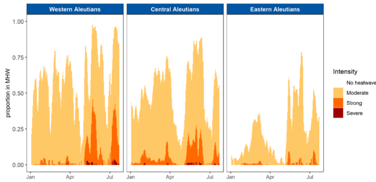
Figure 15: Proportion of region in heatwave status. Heatwave status calculations were performed on each 5 × 5 km grid cell within the Aleutian Islands. This figure shows a five day rolling average of the proportion of cells within each region that are in MHW status. Data extends through August 2022
