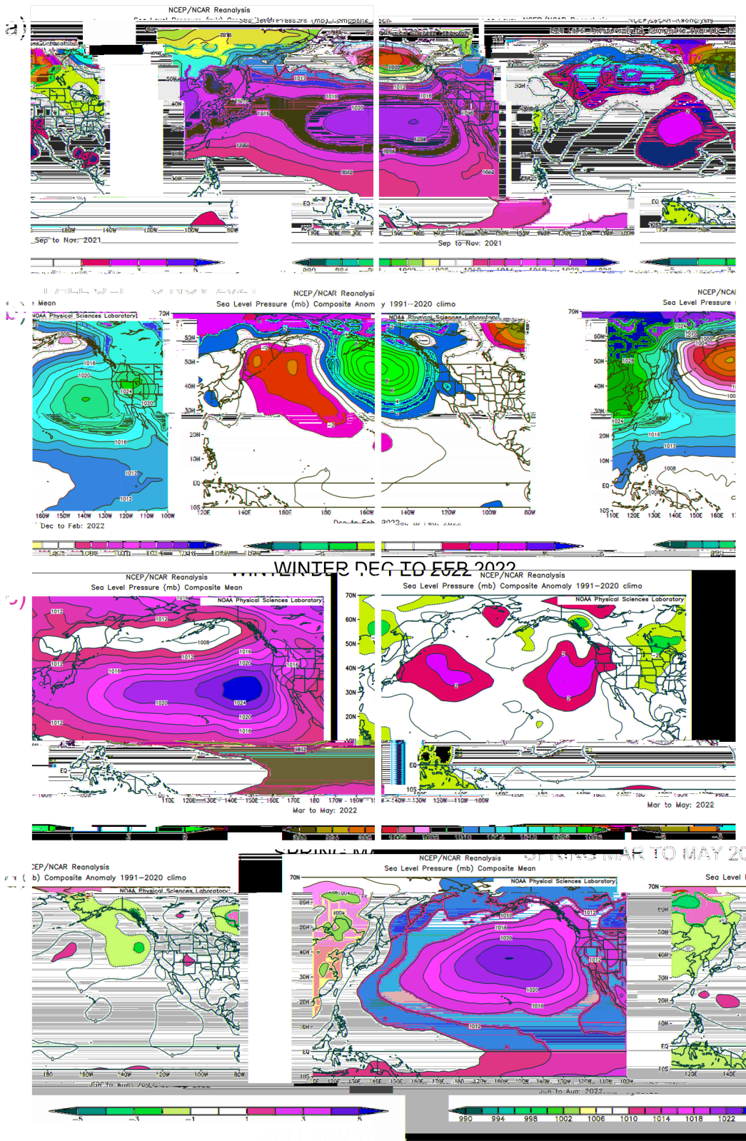
Figure 8: Left, right, Top to bottom: SLP mean and anomalies (hPa) for September–November 2021, December 2021–February 2022, March–May 2022, June–August 2022.
