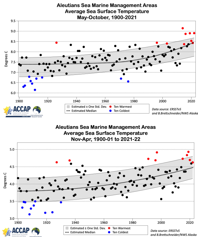
Figure 11: Sea surface temperatures for the Aleutian Islands from 1900–2022 for (a) summer (May–Oct) and (b) winter (Nov–Apr). Presented here are the quantiles representing \pm 1 standard deviation of a Gaussian distribution and for completeness the median calculated using constrained B-Spline regression.
