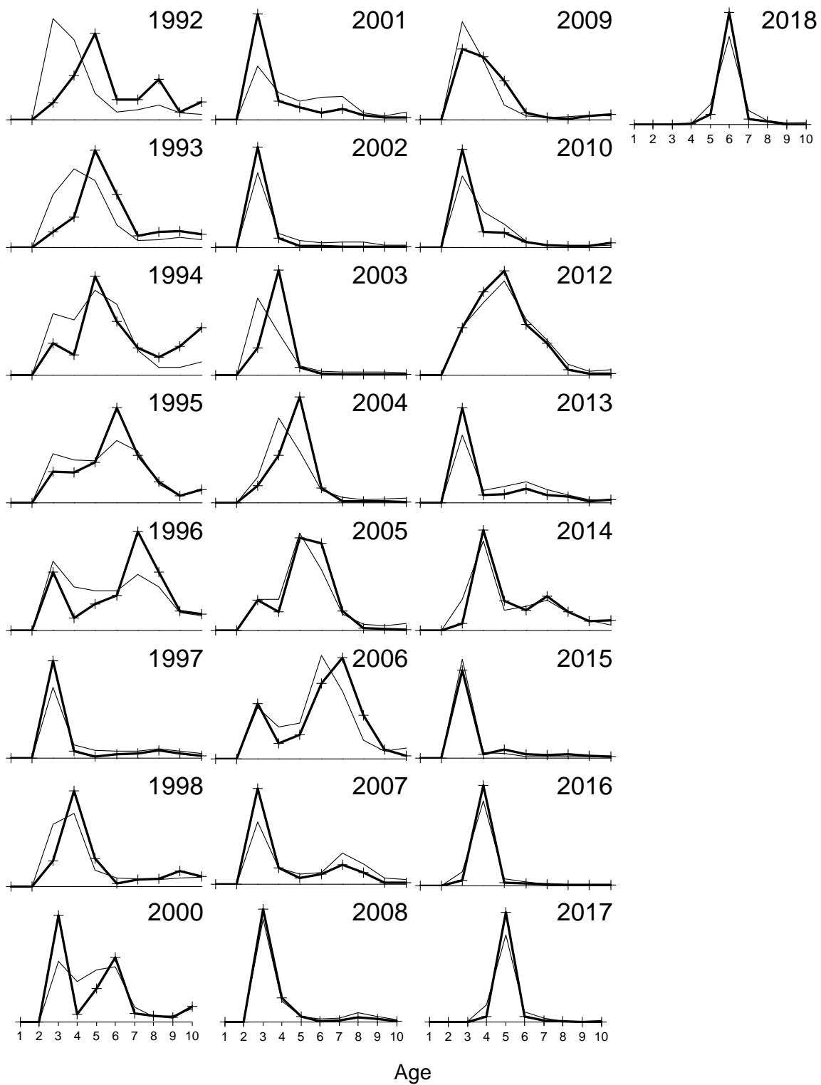
Figure 1.26. Observed and predicted Shelikof Strait acoustic survey age composition for GOA pollock from the base model. Continuous lines are model predictions and lines with + symbol are observed proportions at age.
