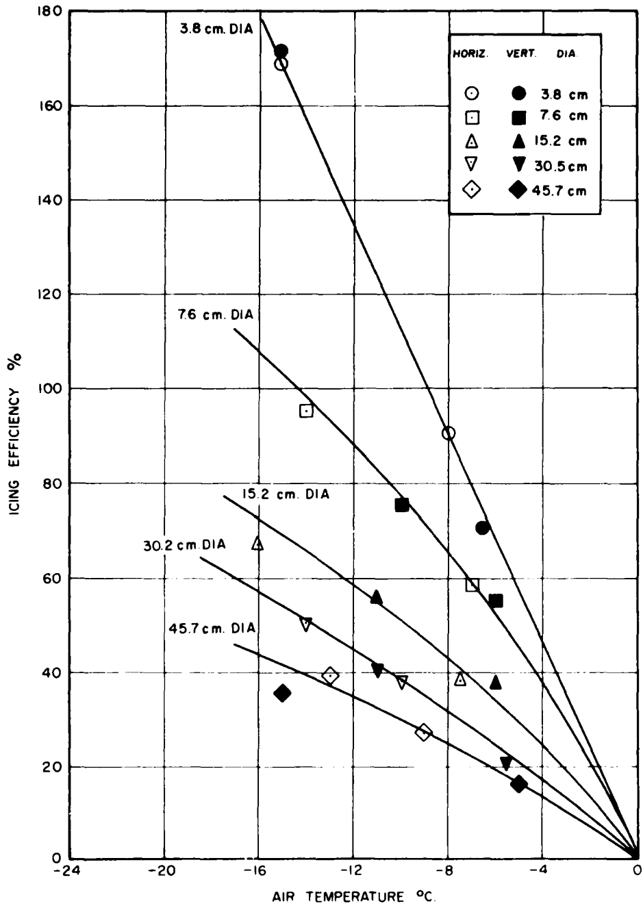
FIG. 5: EFFECT OF TEMPERATURE ON ICING EFFICIENCY
