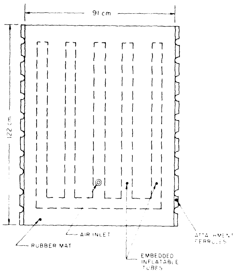
(a) LAYOUT OF PNEUMATIC DE-ICER
