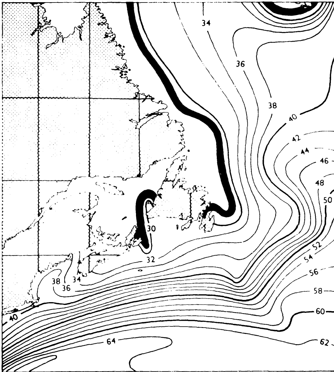
FIG. 17: MEAN SEA-SURFACE TEMPERATURE ( ^{\circ} F) FOR FEBRUARY (FROM OCEANOGRAPHIC ATLAS - REF. 37)
