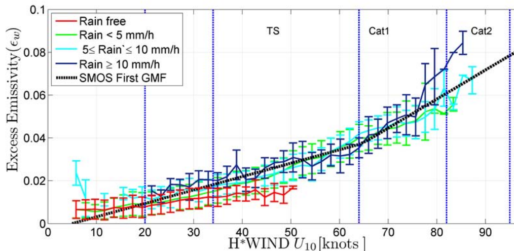
723 Fig. 12: Potential effects of rain on the excess L-band emissivity \Delta e in storm conditions. Top: GMF 724 deduced from the SMOS and H*WIND matchups with rain rate provided from CMORPH=0 (red) and 725 rain rate > 0 (blue). Bottom: similar caption than for the top plot except that the data are now classified 726 by ranges of rain rate (RR): RR=0 (red), 0<RR≤5 mm/h (green), 5mm/h<RR≤10 mm/h (cyan) and 727 RR>10 mm/h. (blue).
