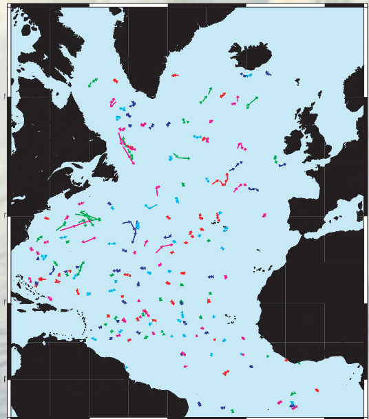
Positions in December 1998 of 190 profiling floats gathering data in the North Atlantic Ocean.
