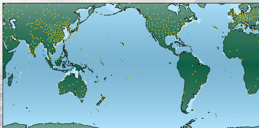
Profiling the atmosphere. A typical network of surface observing stations from which radiosonde balloons (left) collect atmospheric temperature and humidity profiles every 12 hours. An Argo float is the oceanic equivalent of a radiosonde.
