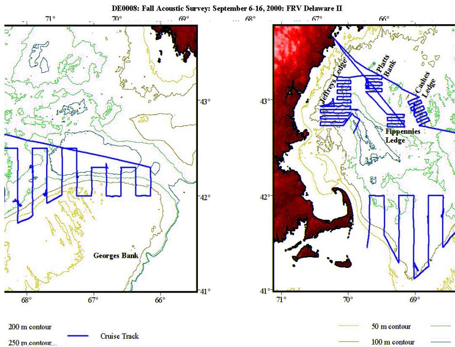
Figure 7.6. Cruise track for systematic parallel surveys conducted on Jeffreys Ledge, Platts Bank, Fippennies Ledge, Cashes Ledge, and Georges Bank during the 2000 Atlantic Herring Hydroacoustic Surveys
