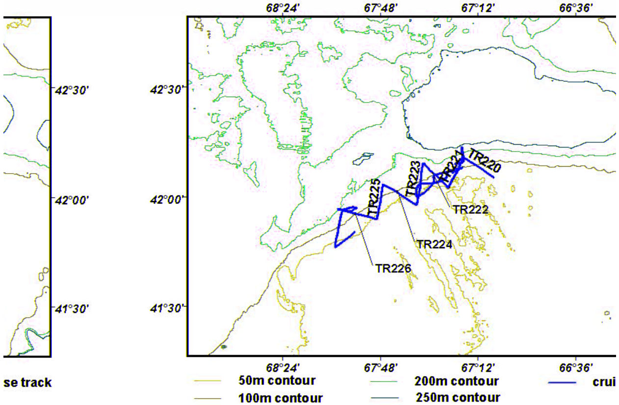
Figure 7.3. Cruise track for one zigzag survey on the northern edge of Georges Bank during the 1998 Atlantic Herring Hydroacoustic Survey.
