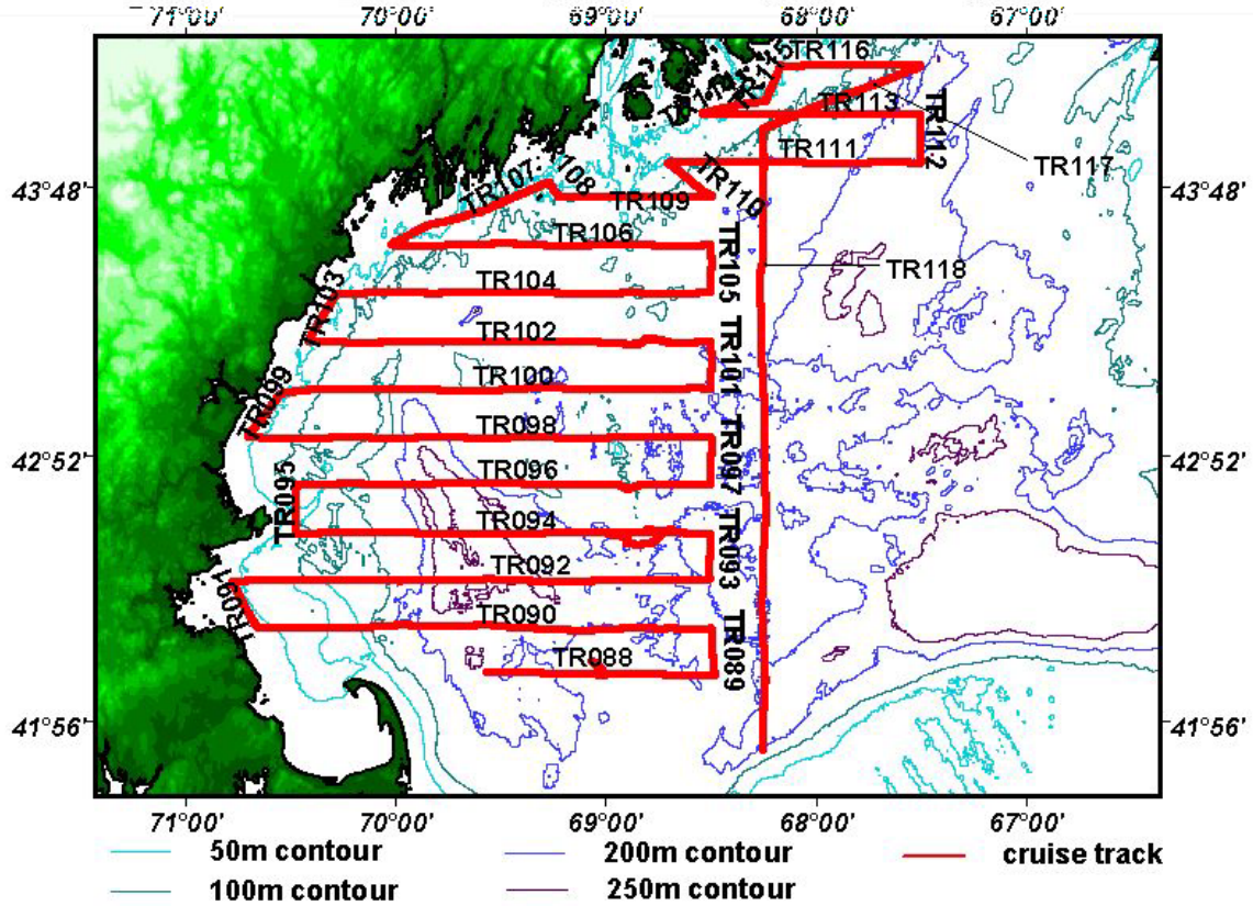
Figure 7.2. Cruise track for the systematic parallel survey (20 nautical miles spacing between transects) in the Gulf of Maine during the 1998 Atlantic Herring Hydroacoustic Survey
