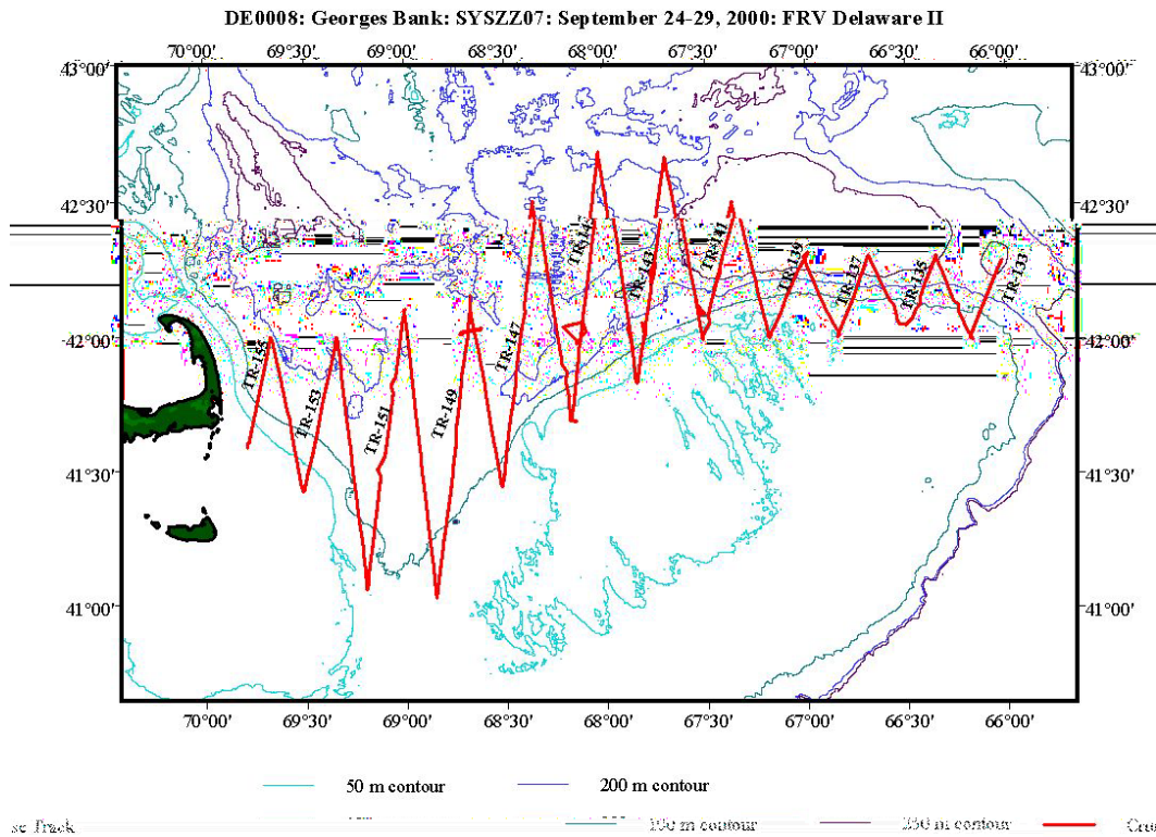
Figure 7.7. Cruise track for the systematic zigzag survey on Georges Bank during 2000.
