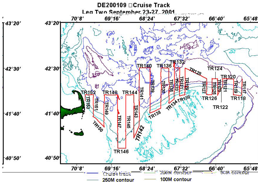
Figure 7.12. Cruise track for the random parallel survey on Georges Bank during the 2001 Atlantic Herring Hydroacoustic Survey.
