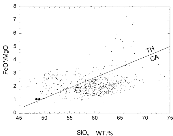
Figure 33. FeO/MgO-silica diagram of Ukinrek Maars volcanic rocks (solid circles) and other Aleutian arc volcanic rocks (small dots) of continental affinity (those located east of 165^\circ\text{W} longitude). Tholeiitic versus calc-alkaline discriminant line from Miyashiro (1974).s.
