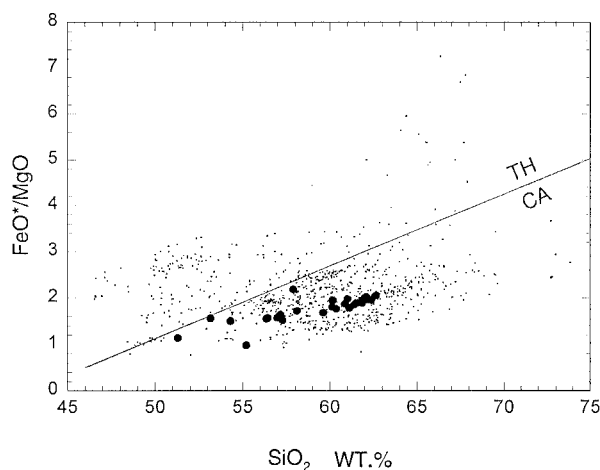
Figure 15. FeO/MgO-silica diagram of Iliamna volcanic rocks (solid circles) and other Aleutian arc volcanic rocks (small dots) of continental affinity (those located east of 165^{\circ}\text{W} longitude). Tholeiitic versus calc-alkaline discriminant line from Miyashiro (1974).
