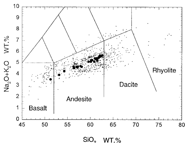
Figure 14. Total alkalis-silica diagram of Iliamna volcanic rocks (solid circles) and other Aleutian arc volcanic rocks (small dots) of continental affinity (those located east of 165^{\circ}\text{W} longitude). Discriminant lines and field names (Le Bas and others, 1986) are explained on Figure 2.
