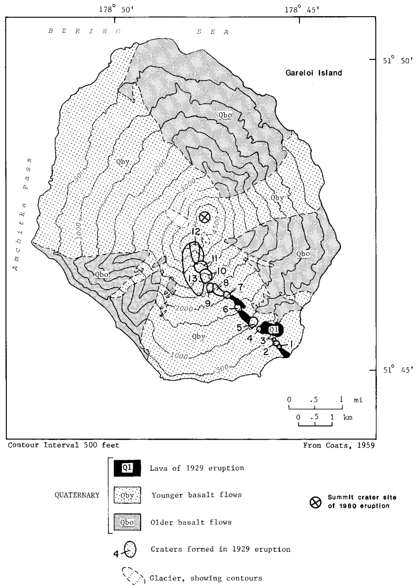
Figure 93. Geologic map of Gareloi Island after Coats (1959).
