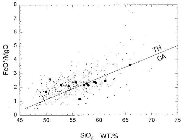
Figure 88. \text{FeO}/\text{MgO} -silica diagram of Great Sitkin volcanic rocks (solid circles) and other Aleutian arc volcanic rocks (small dots) of oceanic affinity (those located west of 165^\circ\text{W} longitude). Tholeiitic versus calc-alkaline discriminant line from Miyashiro (1974).
