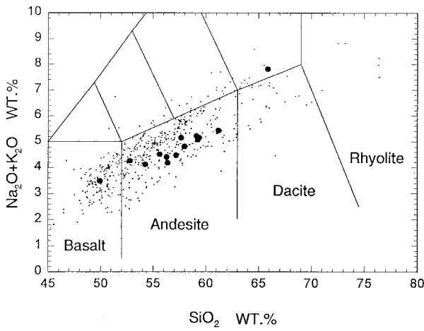
Figure 87. Total alkalis-silica diagram of Great Sitkin volcanic rocks (solid circles) and other Aleutian arc volcanic rocks (small dots) of oceanic affinity (those located west of 165^\circ\text{W} longitude). Discriminant lines and field names (Le Bas and others, 1986) are explained on Figure 2.
