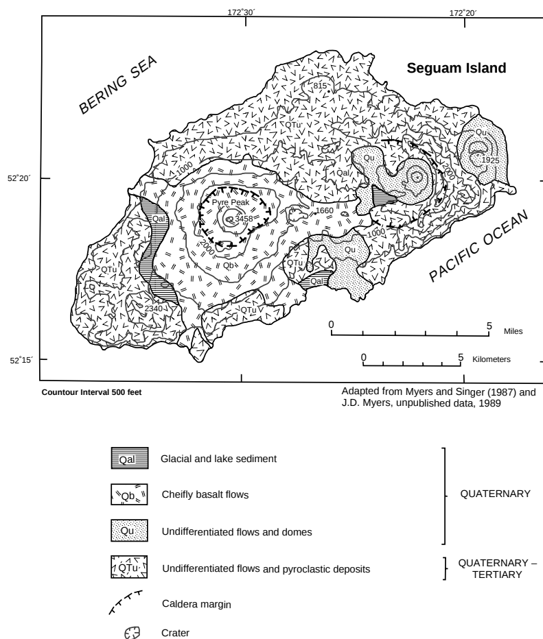
Figure 77. Geologic map of Seguam Island modified from Myers and Singer (1987) and J.D. Myers, unpublished data, 1989.
