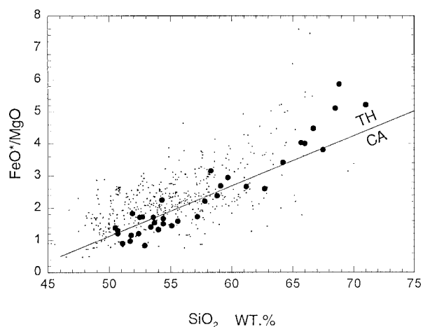
Figure 79. \text{FeO}^*/\text{MgO} -silica diagram of Sequam volcanic rocks (solid circles) and other Aleutian arc volcanic rocks (small dots) of oceanic affinity (those located west of 165°W longitude). Tholeiitic versus calc-alkaline discriminant line from Miyashiro (1974).
