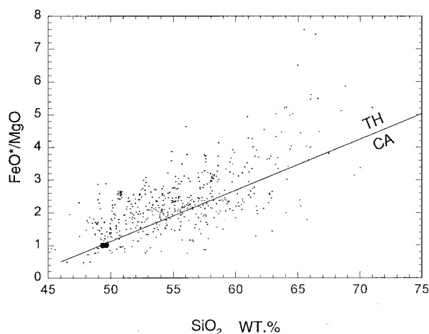
Figure 85. \text{FeO}^*/\text{MgO} -silica diagram of Kasatochi volcanic rocks (solid circles) and other Aleutian arc volcanic rocks (small dots) of oceanic affinity (those located west of 165°W longitude). Tholeiitic versus calc-alkaline discriminant line from Miyashiro (1974).
