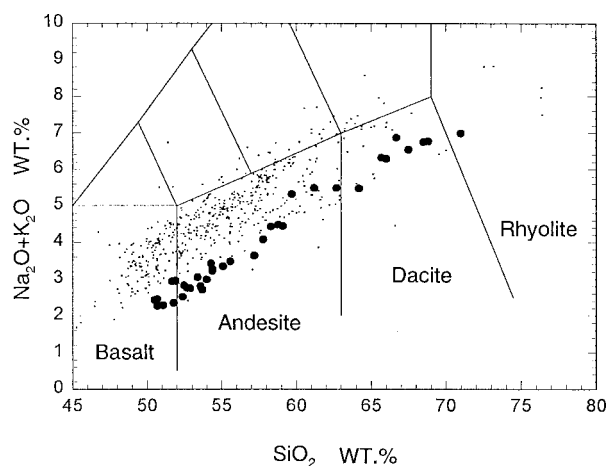
Figure 78. Total alkalis-silica diagram for Sequam volcanic rocks (solid circles) and other Aleutian arc volcanic rocks (small dots) of oceanic affinity (those located west of 165°W longitude). Discriminant lines and fieldnames (LeBas and others, 1986) are explained in Figure 2.
