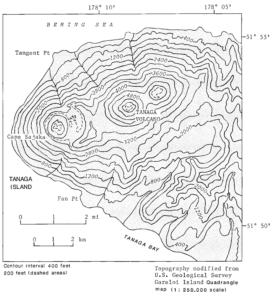
Figure 92. Topographic map of Tanaga volcano.
