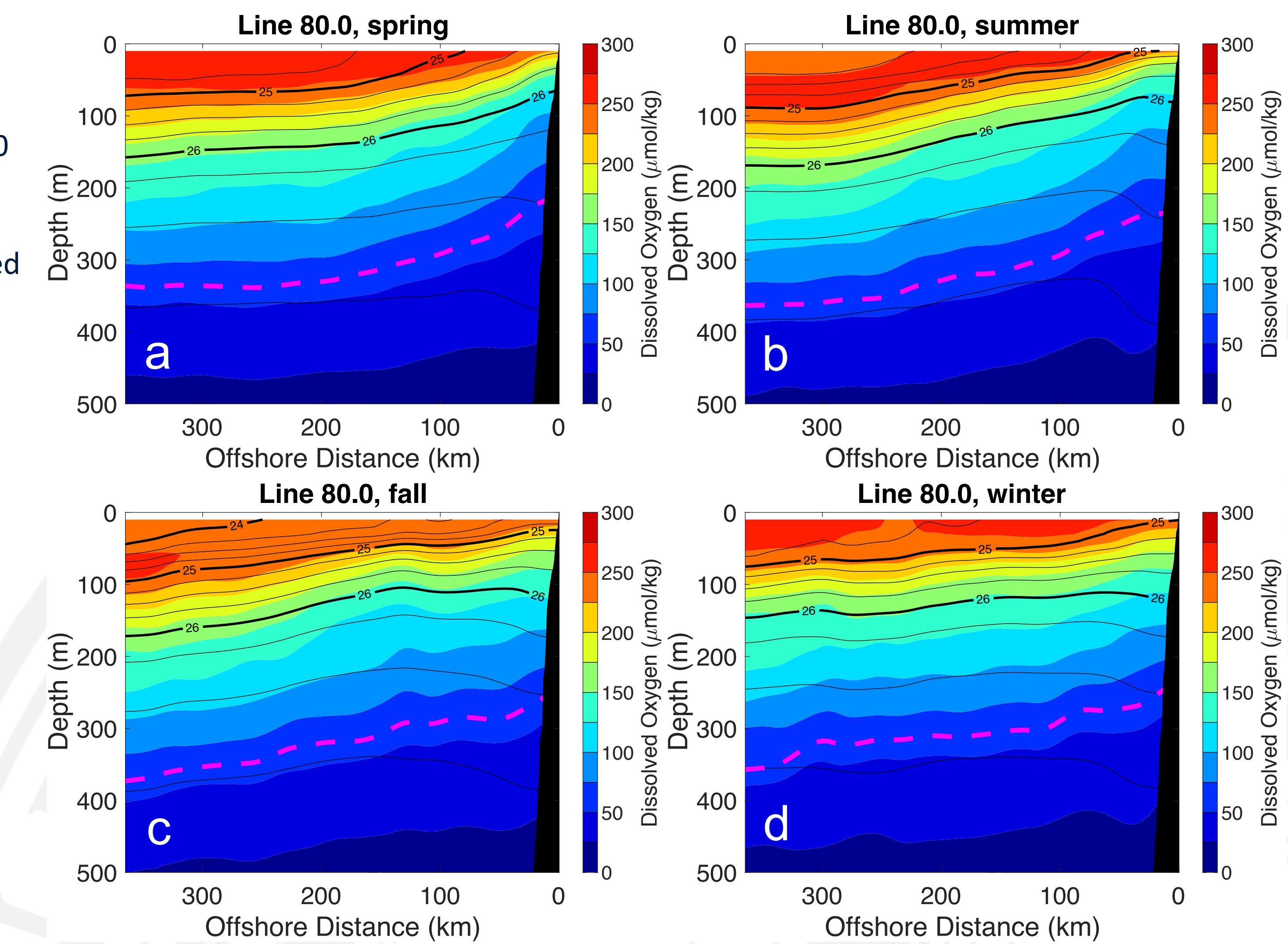
Seasonal plots of dissolved oxygen on Line 80.0. (a) Spring (b) summer (c) fall and (d) winter. The winter season is defined as December through February. Thin black lines denote potential density surfaces. Thick black lines denote \sigma_\theta 24 kg m -3 , 25 kg m -3 , and 26 kg m -3 . A hypoxic boundary of 60 umol kg -1 is plotted in a dashed magenta line.
