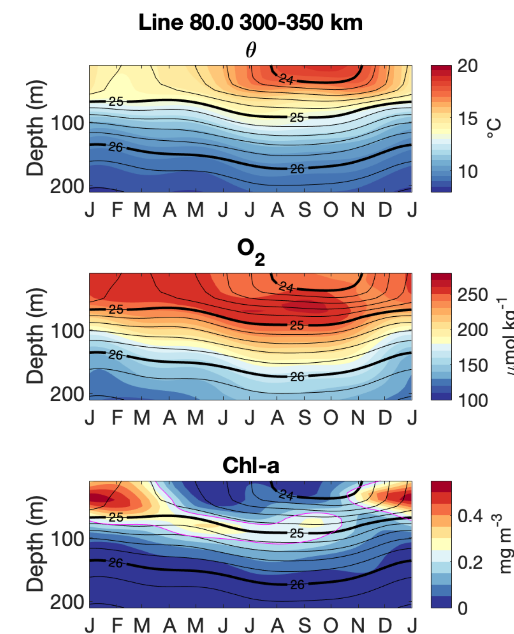
Seasonal temperature, dissolved oxygen concentration, and chl-a concentration over the top 200 m on line 80.0, averaged from 300-350 km from shore. Black lines indicate potential density surfaces. The thin magenta line denotes the 0.2 mg m -3 chl-a contour.
