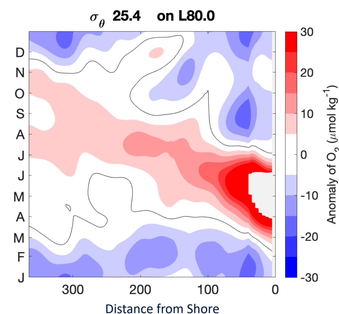
Seasonal anomaly of dissolved oxygen from the mean on potential density surface 25.4 kg m -3 . The grey region April-May indicates that the isopycnal has outcropped.
