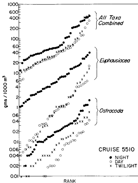
Figure 2. Scatter diagram of three representative examples showing the distribution of biomass ranked in order of increasingly higher values. Each set of data consists of all measurements of a functional group derived from a single cruise. Day, twilight and night samples are differentiated and the scale of ranked position (abscissa) is adjusted so that the number of samples per time period extends over the same length irrespective of the number of observations. Further comments in the text.
