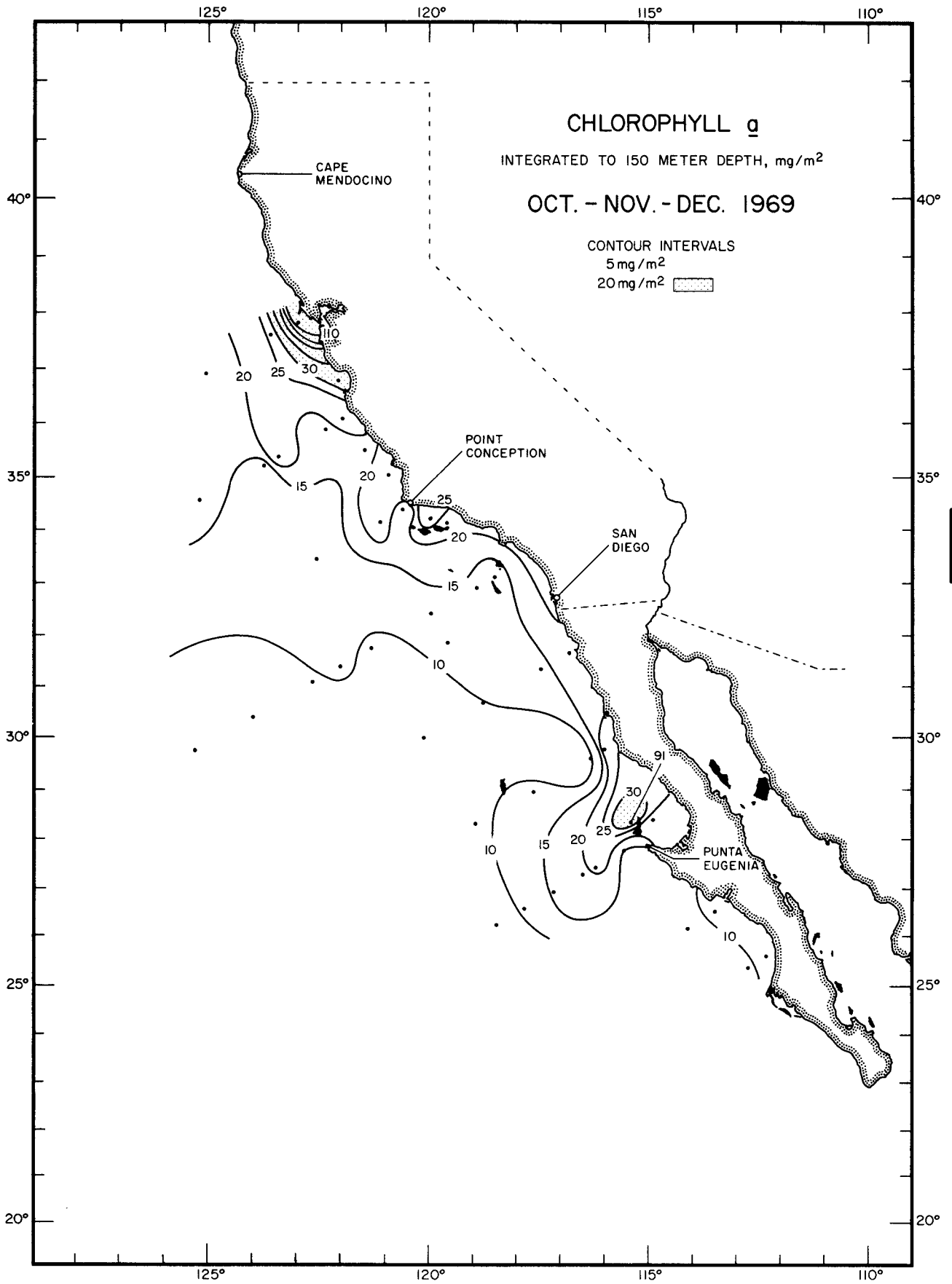
CHLOROPHYLL a INTEGRATED OCT. - NOV. - DEC. 1969
