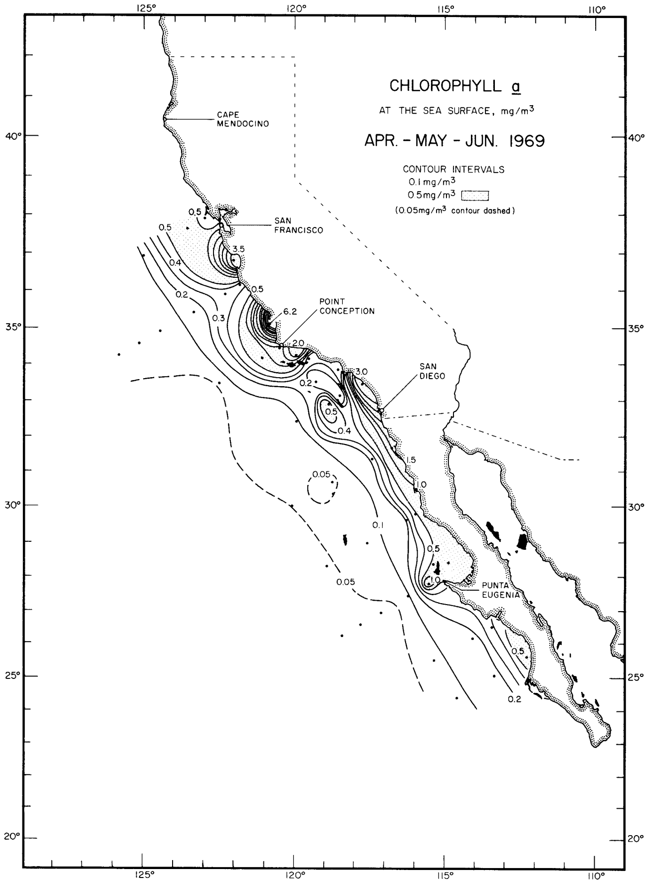
CHLOROPHYLL a SURFACE APR. - MAY - JUN. 1969
