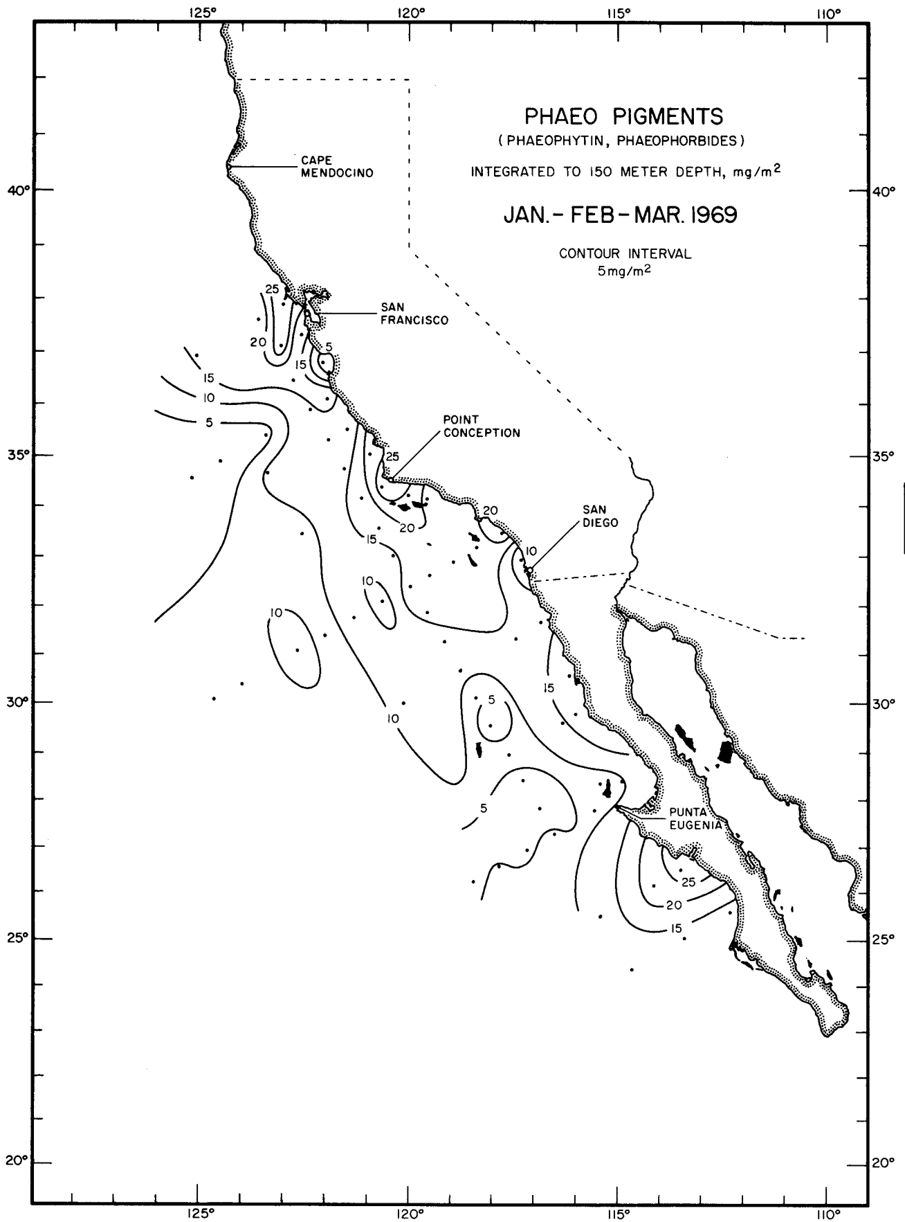
PHAEO PIGMENTS JAN. - FEB. - MAR. 1969
