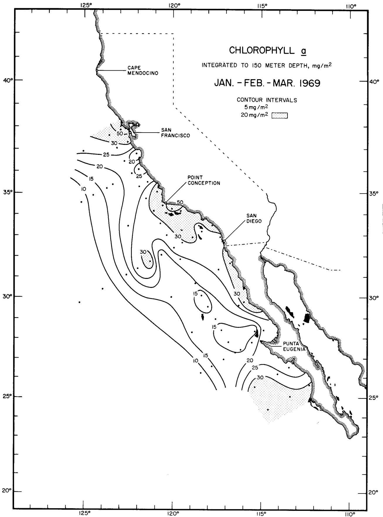
CHLOROPHYLL a INTEGRATED JAN. - FEB. - MAR. 1969
