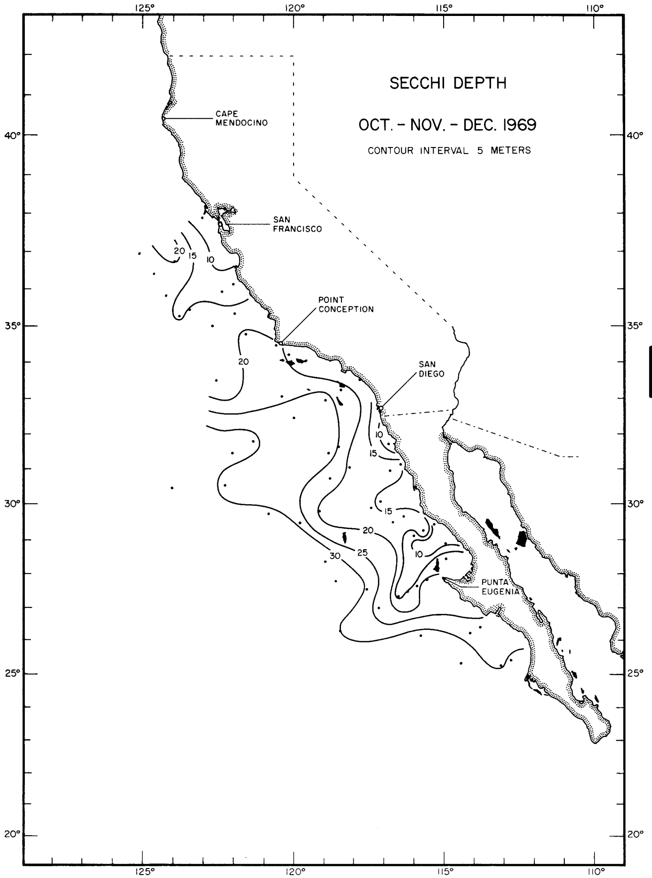
SECCHI DEPTH OCT. - NOV. - DEC. 1969
