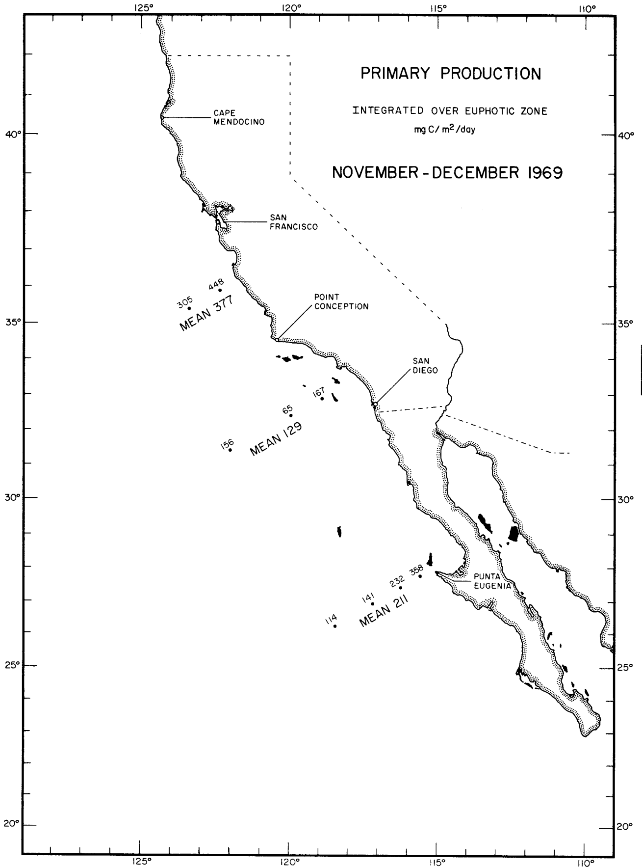
PRIMARY PRODUCTION NOVEMBER - DECEMBER 1969
