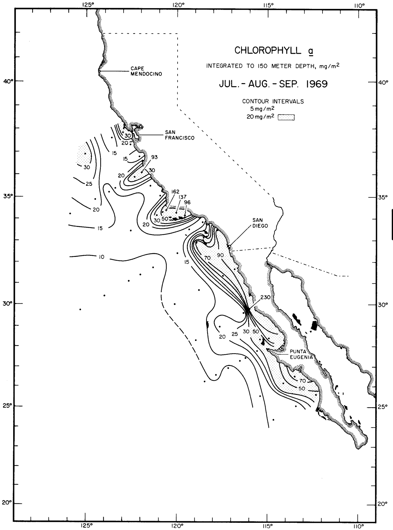
CHLOROPHYLL a INTEGRATED JUL. - AUG. - SEP. 1969
