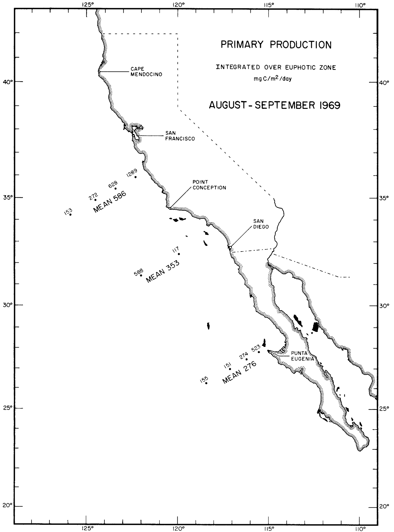
PRIMARY PRODUCTION AUGUST - SEPTEMBER 1969
