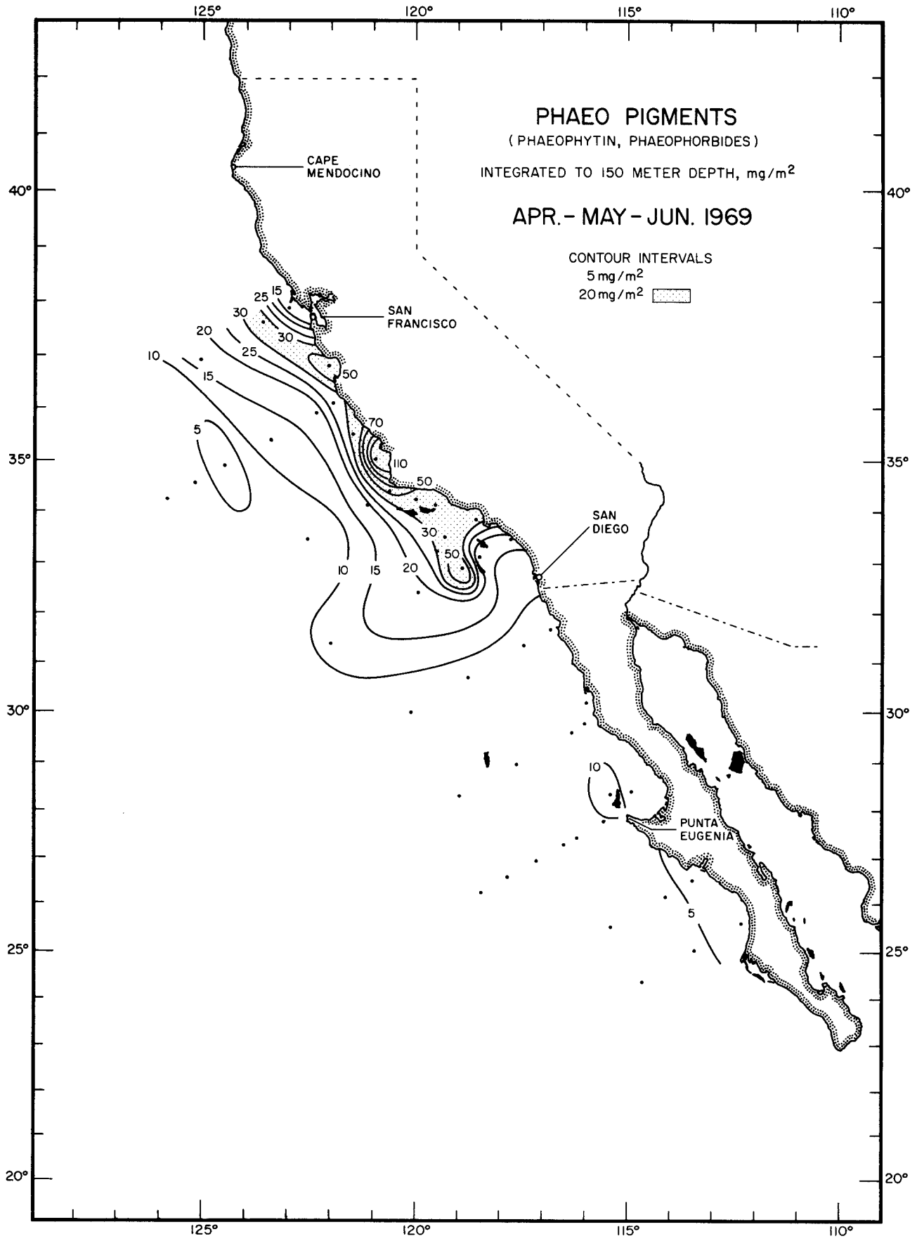
PHAEO PIGMENTS APR. - MAY - JUN. 1969
