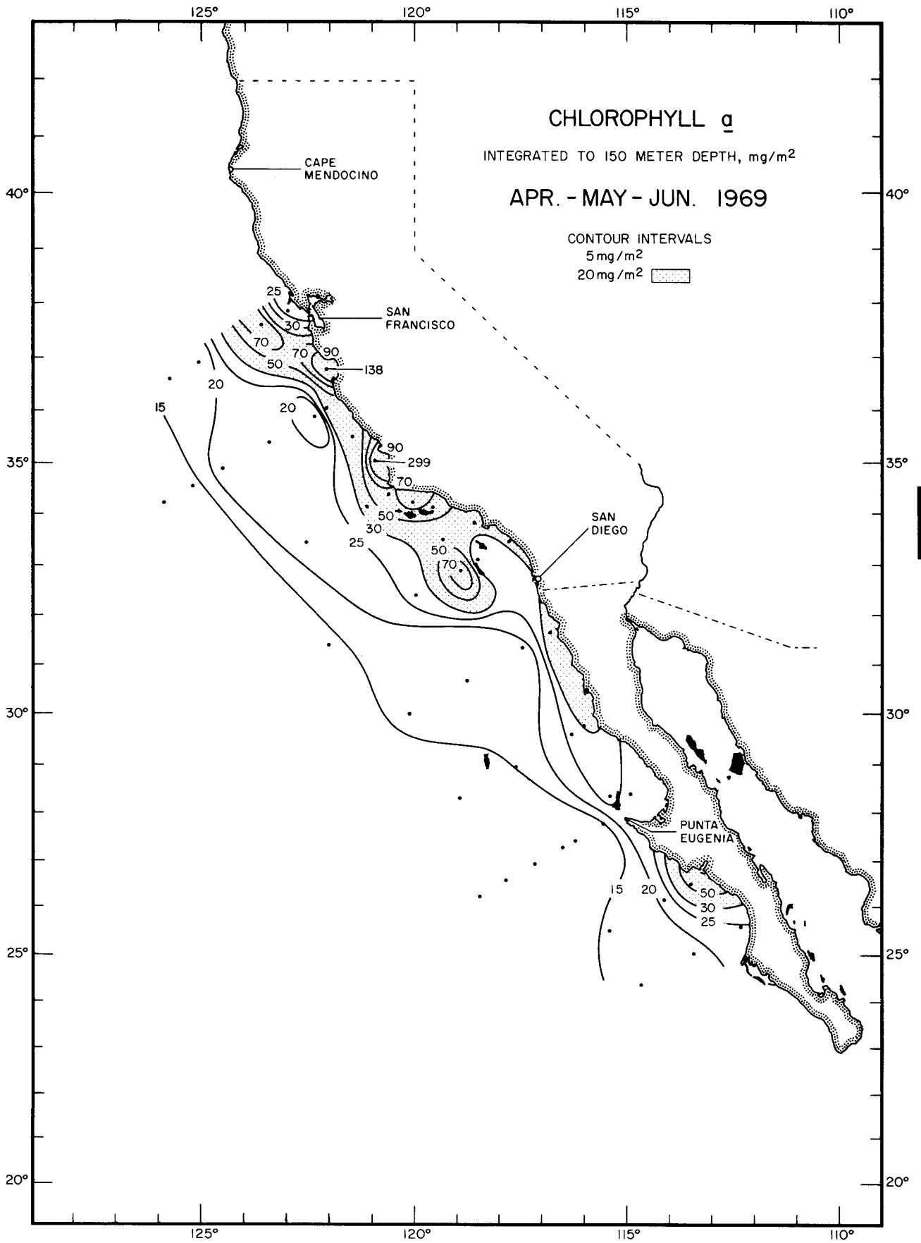
CHLOROPHYLL a INTEGRATED APR. - MAY - JUN. 1969
