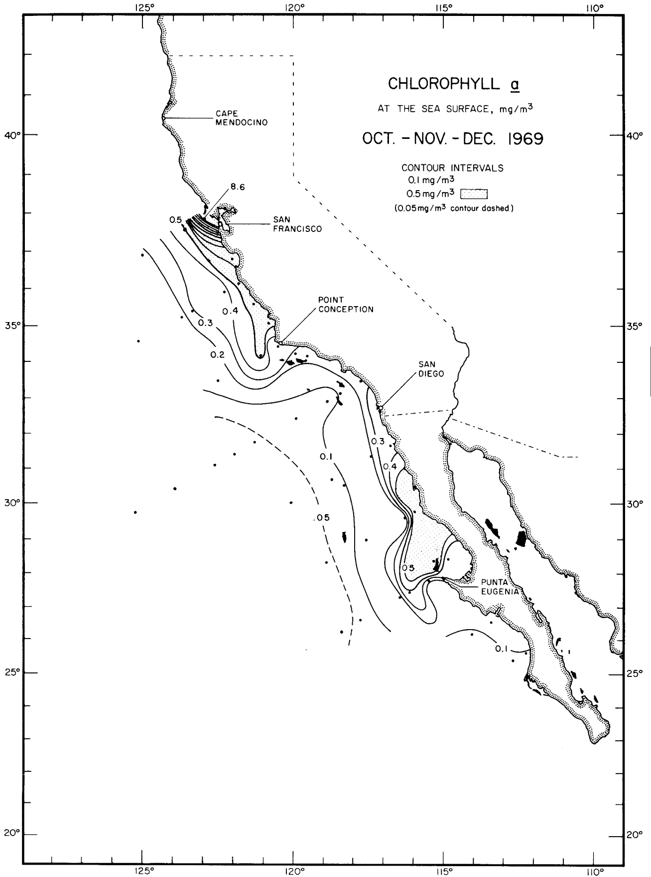
CHLOROPHYLL a SURFACE OCT. - NOV. - DEC. 1969
