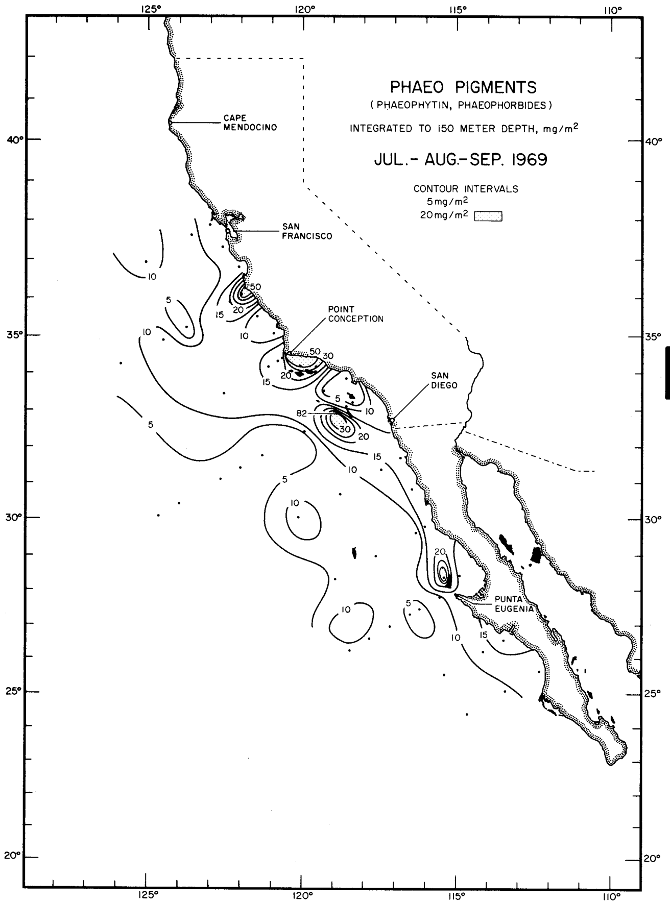
PHAEO PIGMENTS JUL. - AUG. - SEP. 1969
