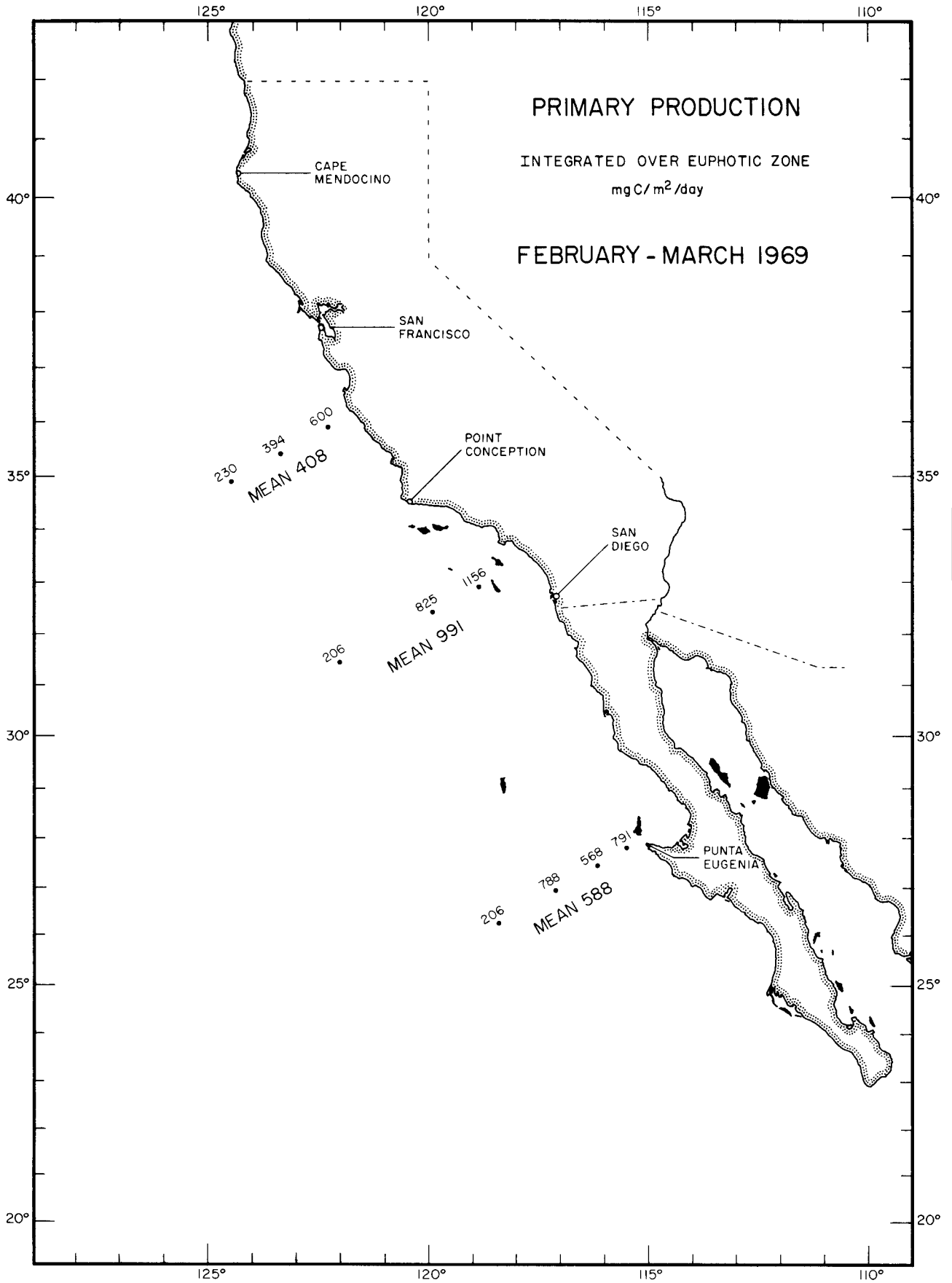
PRIMARY PRODUCTION FEBRUARY - MARCH 1969
