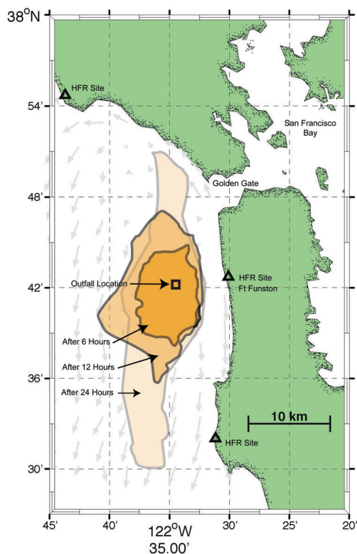
Figure 6: Trajectory forecasts during the Ocean Beach Outfall near San Francisco derived from near-real-time HFR data.
