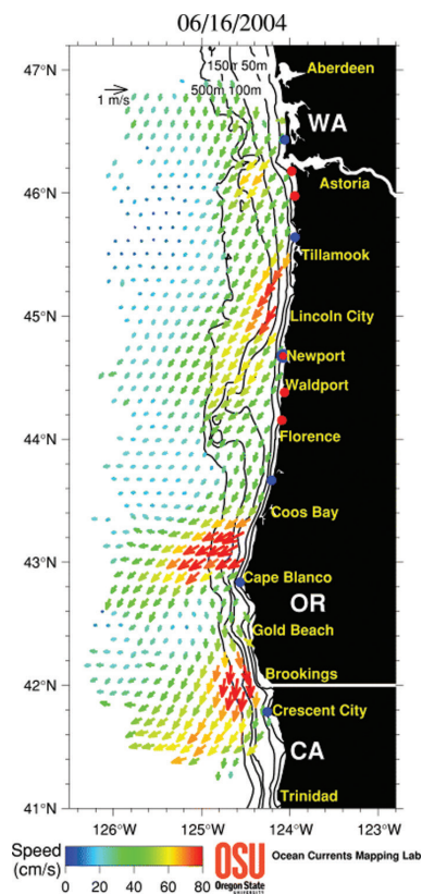
Figure 2: Complex regional coastal flows can only be captured by HFR surface current mapping networks
