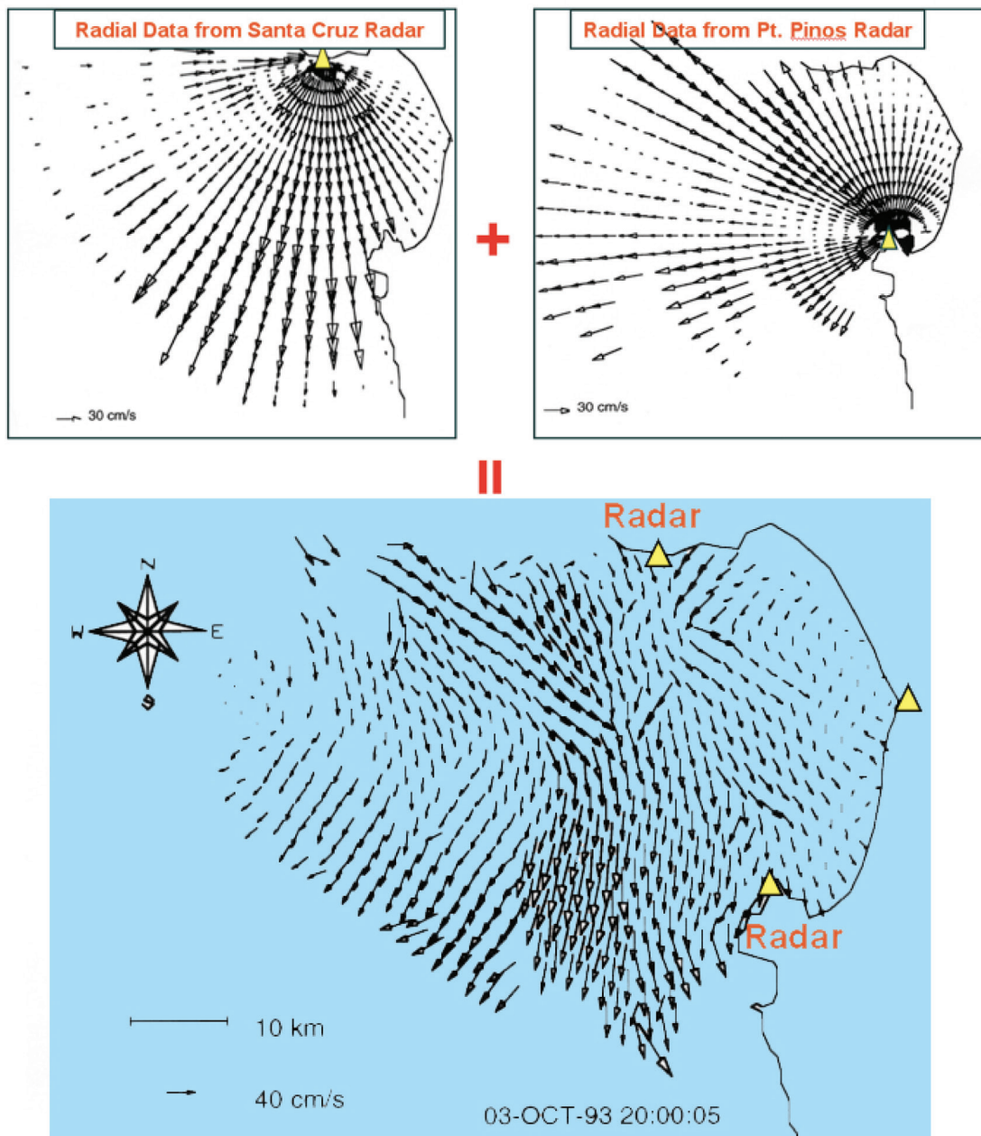
Figure A-3: Radial Velocity Maps from Two HFR Sites and Map of Combined Radials to Create Total Vector Velocity Maps
