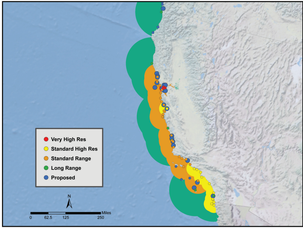
Figure F5: – Full Buildout Illustrating Existing and Proposed HFR Sites for Southwestern United States
