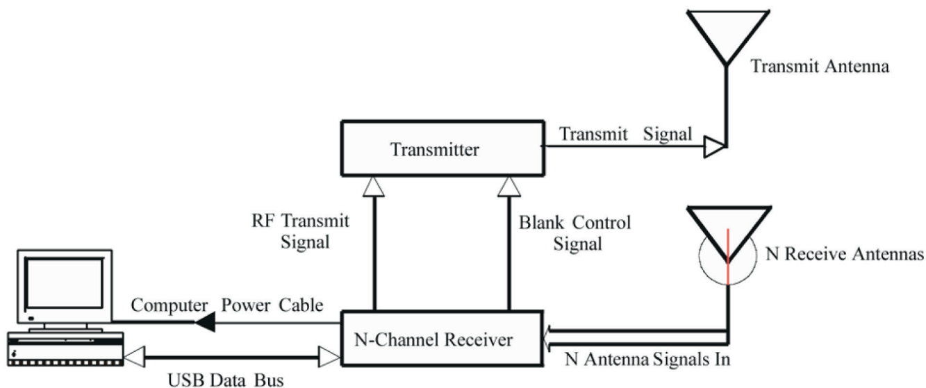
Figure A-2: Diagram of Core HFR Components and Data Flow
