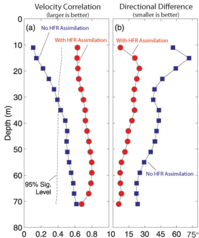
Figure 7: Improvement in model current estimation after assimilating HFR data (from Oke et al., 2002).
