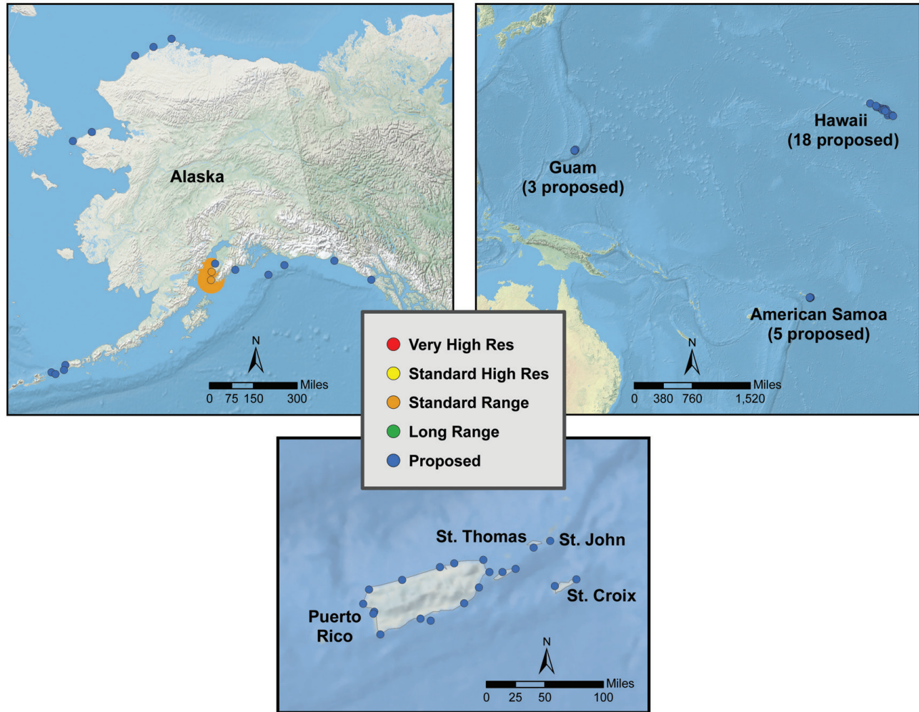
Figure F1: Full Buildout Illustrating Existing and Proposed HFR Sites for Alaska, Pacific Islands, and Caribbean Regions
