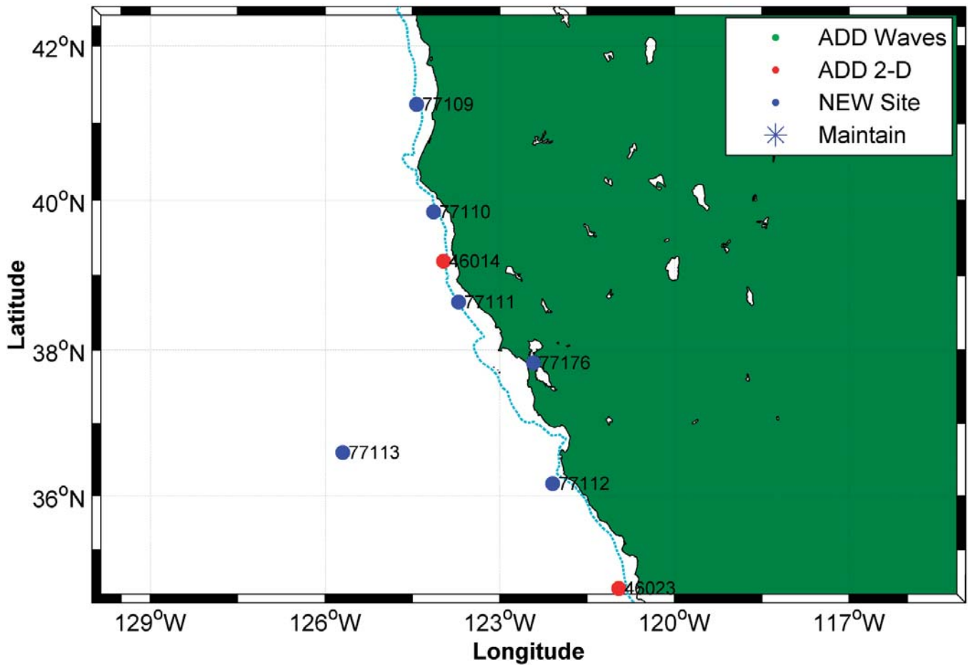
Figure B8. Upgrades to existing and new (70000 series station numbers) wave measurement sites for the Central and Northern California Ocean Observing System, 200-m bottom contour plotted in cyan.
