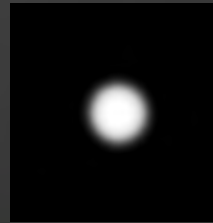
Blinn-Phong
