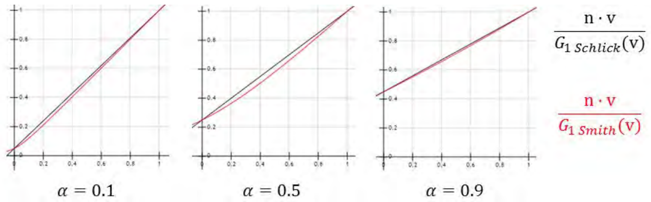
Figure 2: Schlick with k = \alpha/2 matches Smith very closely
