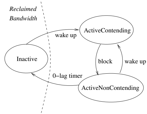
Figure 1: Task state diagram in GRUB.
