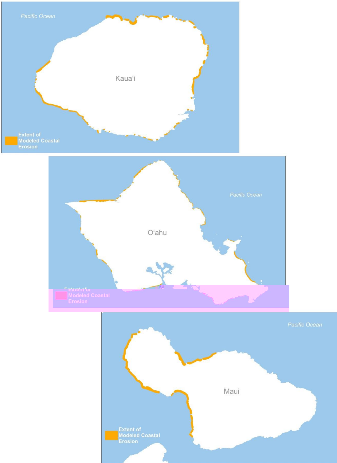
Figure 27. Extent of modeled coastal erosion on Kaua'i, O'ahu, and Maui
