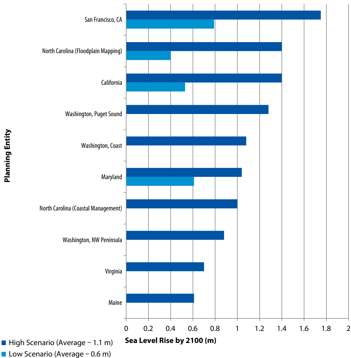
Figure 1: Sea Level Change Scenarios Used by Various State Planning Entities as of 2011.
