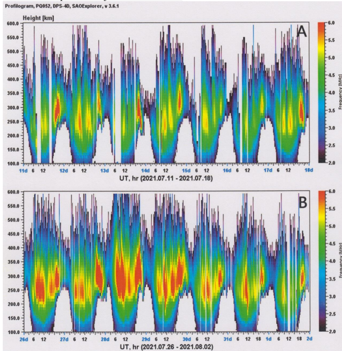
Fig. 13. Profilograms obtained from full electron concentration profiles (manually scaled ionograms) for a cyclonic event (A) and polar front jet stream (B). Profilograms indicate that ionization within the whole F-layer ionosphere is higher during the jet stream event on 29 July 2021 (B) than ionization around mid-July 2021 (A). In both cases, oscillations in the gravity wave domain are well observed during the entire studied time span.
