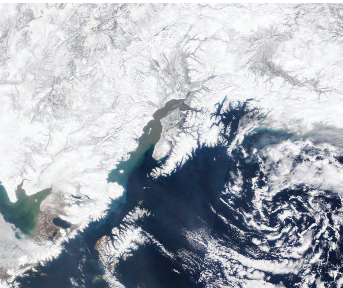
Alaska from MODIS instrument aboard NASA's Terra satellite, 30 Mar 2018
