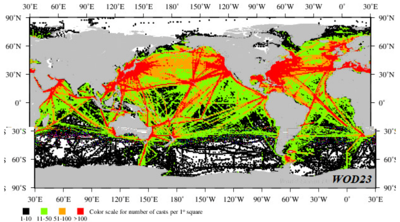
Figure 4.1. Geographic distribution of XBT profiles in WOD23: number of profiles by one-degree squares.
